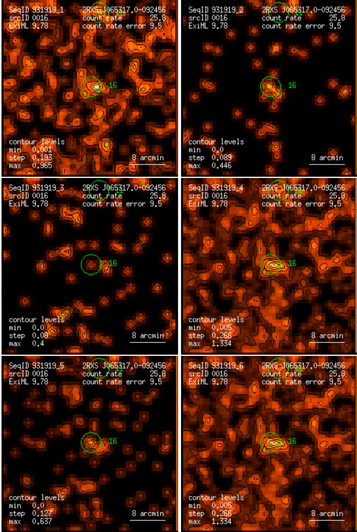
Figure 16: RASS 931919: detection 0016: band rate images, Gaussian filter: (1) PSPC channels 11 – 41, (2) 52 – 90, (3) 91 – 201, (4) 11 – 235, (5) 52 – 201, (6) 11 – 201. Broad band rates in counts/ks. Band rate contour levels in counts/ks/arcmin 2 .
