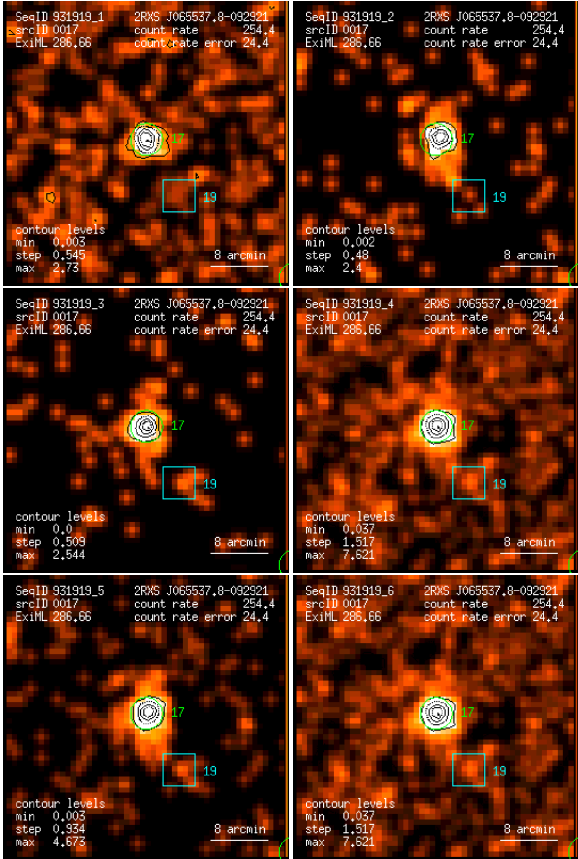
Figure 17: RASS 931919: detection 0017: band rate images, Gaussian filter: (1) PSPC channels 11 – 41, (2) 52 – 90, (3) 91 – 201, (4) 11 – 235, (5) 52 – 201, (6) 11 – 201. Broad band rates in counts/ks. Band rate contour levels in counts/ks/arcmin 2 .
