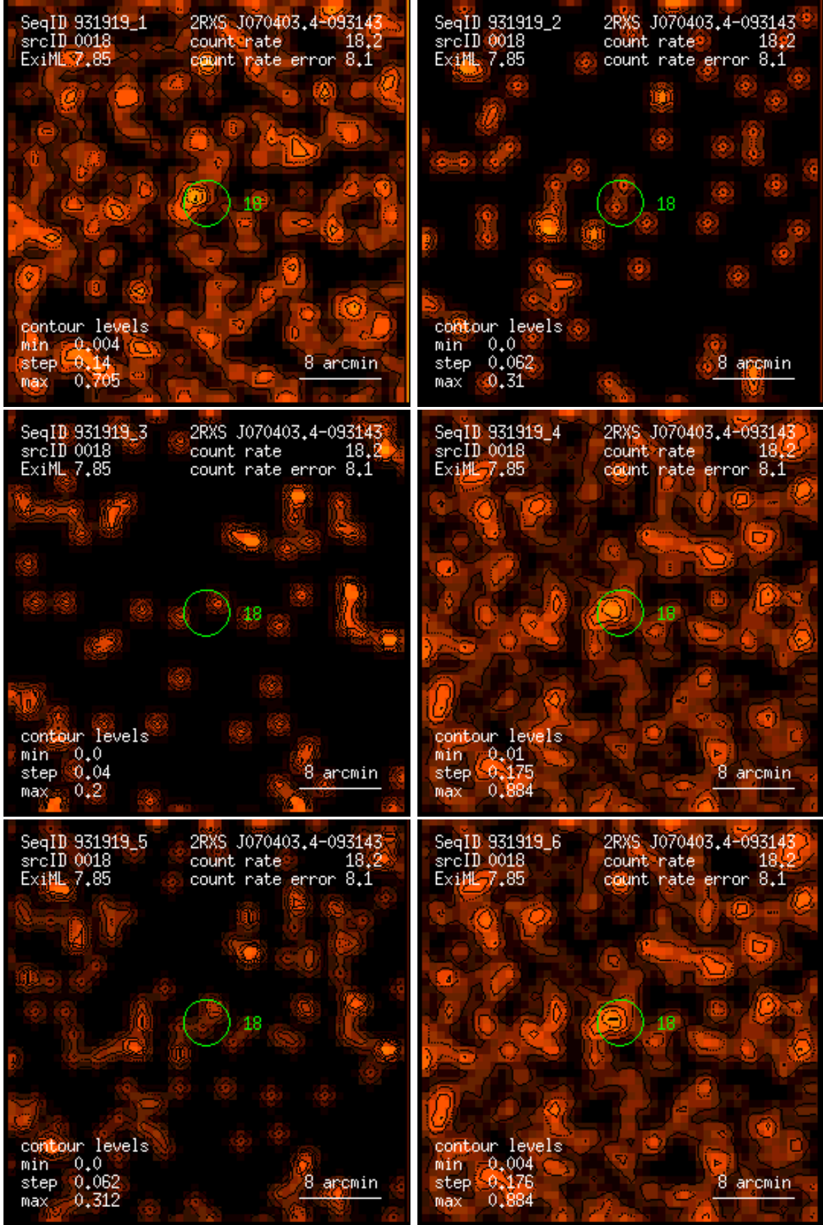
Figure 18: RASS 931919: detection 0018: band rate images, Gaussian filter: (1) PSPC channels 11 – 41, (2) 52 – 90, (3) 91 – 201, (4) 11 – 235, (5) 52 – 201, (6) 11 – 201. Broad band rates in counts/ks. Band rate contour levels in counts/ks/arcmin 2 .
