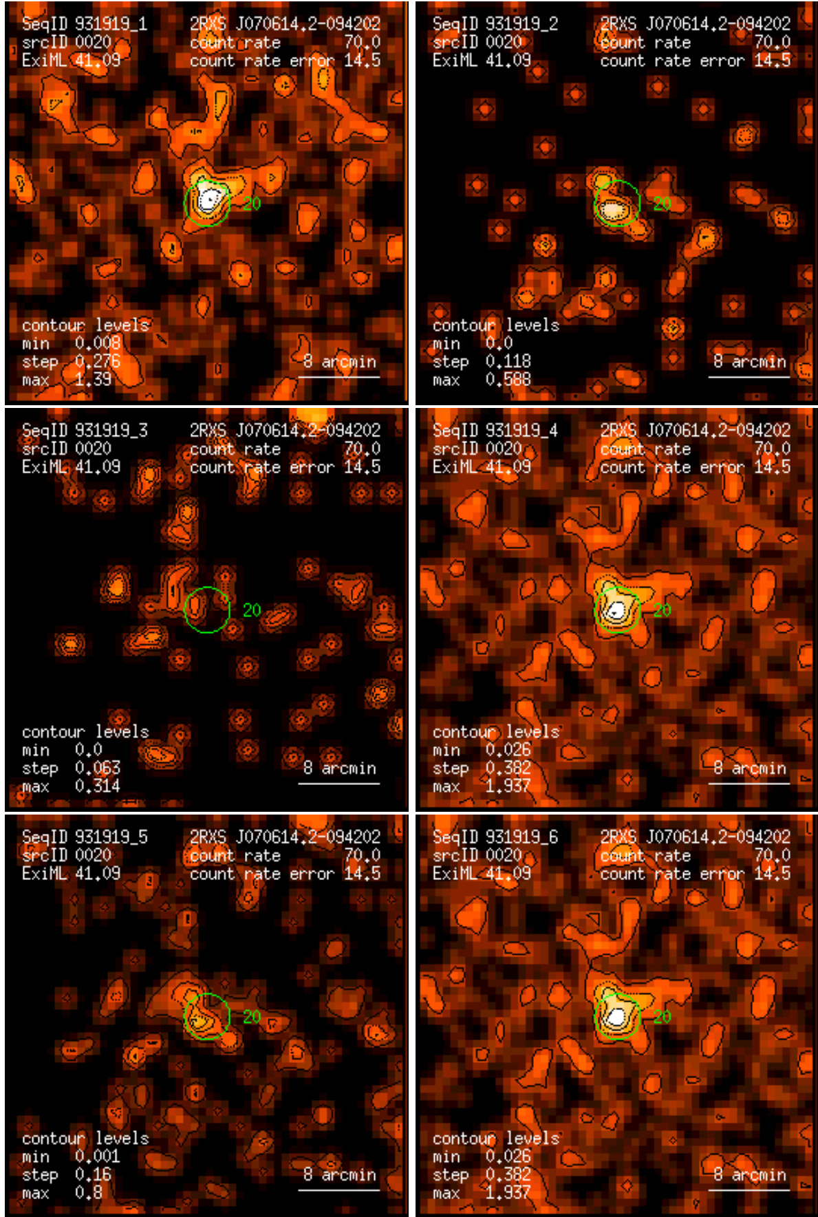
Figure 20: RASS 931919: detection 0020: band rate images, Gaussian filter: (1) PSPC channels 11 – 41, (2) 52 – 90, (3) 91 – 201, (4) 11 – 235, (5) 52 – 201, (6) 11 – 201. Broad band rates in counts/ks. Band rate contour levels in counts/ks/arcmin 2 .
