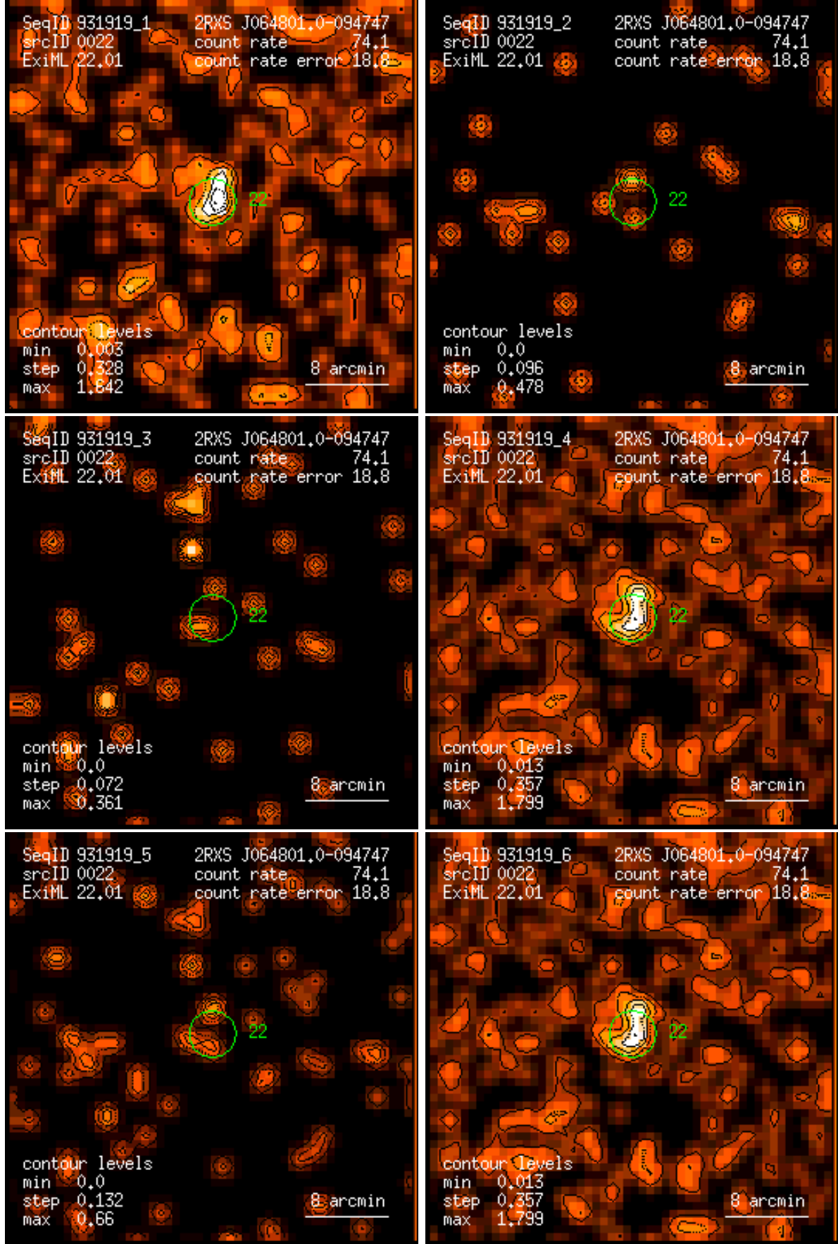
Figure 22: RASS 931919: detection 0022: band rate images, Gaussian filter: (1) PSPC channels 11 – 41, (2) 52 – 90, (3) 91 – 201, (4) 11 – 235, (5) 52 – 201, (6) 11 – 201. Broad band rates in counts/ks. Band rate contour levels in counts/ks/arcmin 2 .
