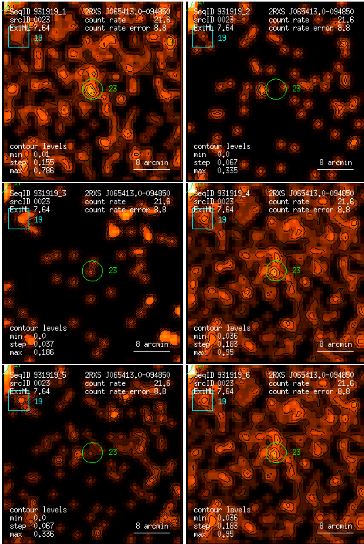
Figure 23: RASS 931919: detection 0023: band rate images, Gaussian filter: (1) PSPC channels 11 – 41, (2) 52 – 90, (3) 91 – 201, (4) 11 – 235, (5) 52 – 201, (6) 11 – 201. Broad band rates in counts/ks. Band rate contour levels in counts/ks/arcmin 2 .
