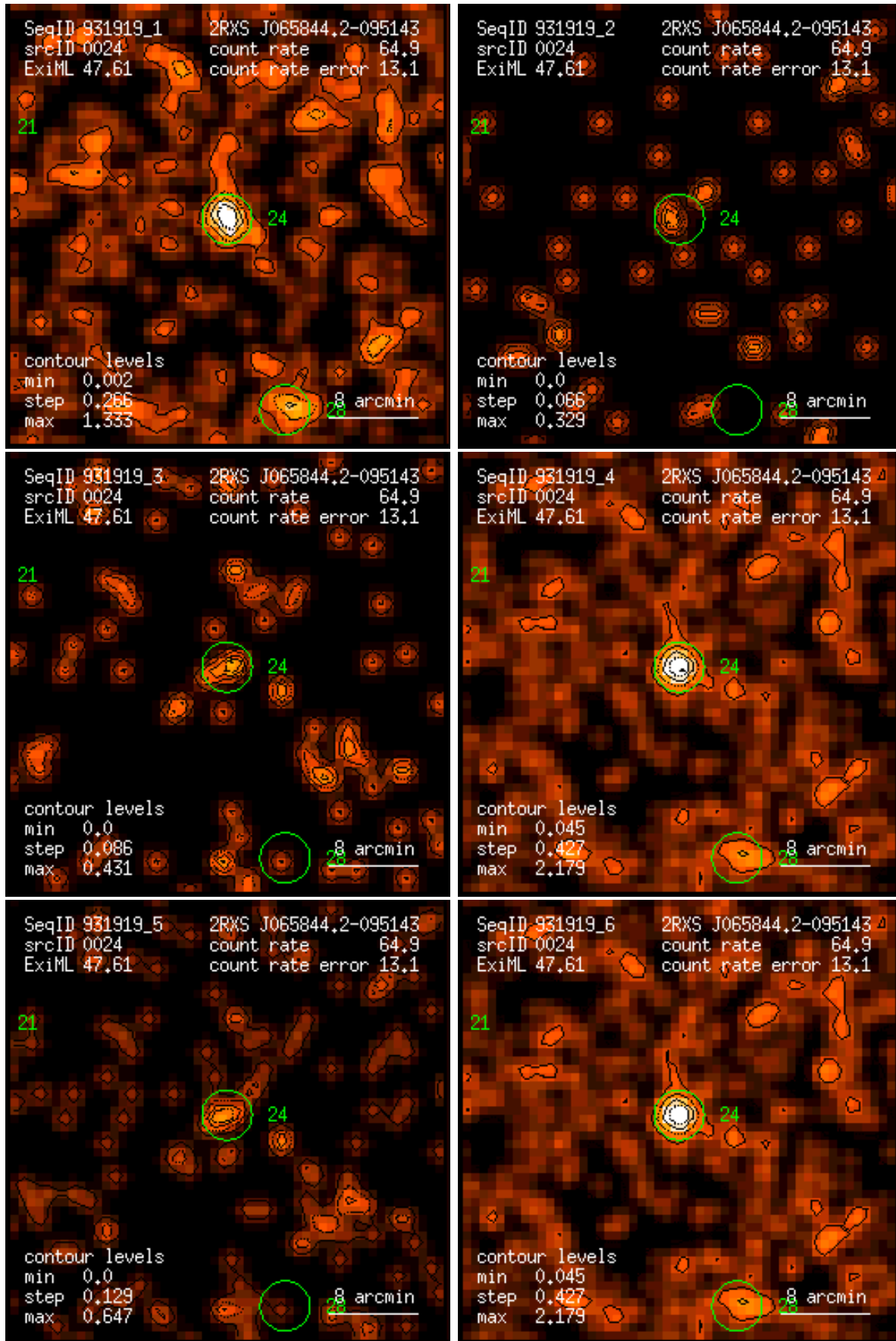
Figure 24: RASS 931919: detection 0024: band rate images, Gaussian filter: (1) PSPC channels 11 – 41, (2) 52 – 90, (3) 91 – 201, (4) 11 – 235, (5) 52 – 201, (6) 11 – 201. Broad band rates in counts/ks. Band rate contour levels in counts/ks/arcmin 2 .
