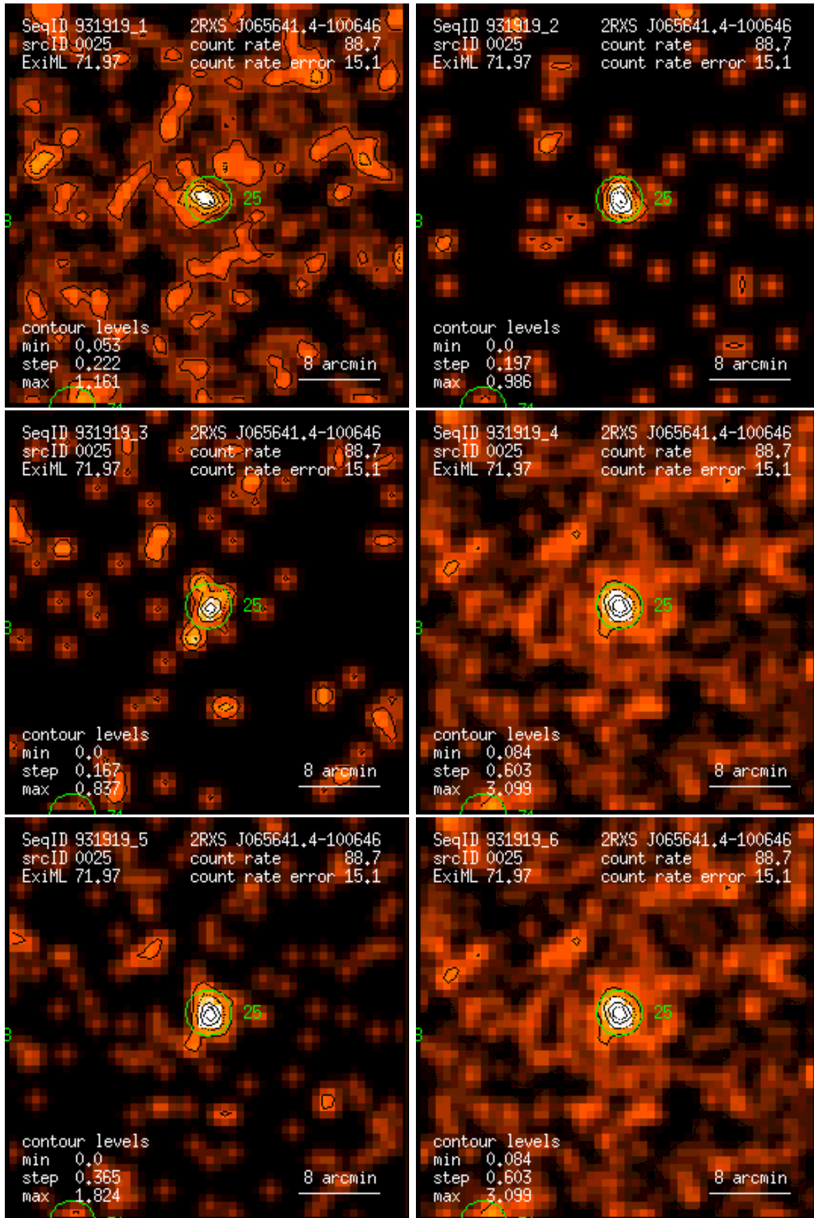
Figure 25: RASS 931919: detection 0025: band rate images, Gaussian filter: (1) PSPC channels 11 – 41, (2) 52 – 90, (3) 91 – 201, (4) 11 – 235, (5) 52 – 201, (6) 11 – 201. Broad band rates in counts/ks. Band rate contour levels in counts/ks/arcmin 2 .
