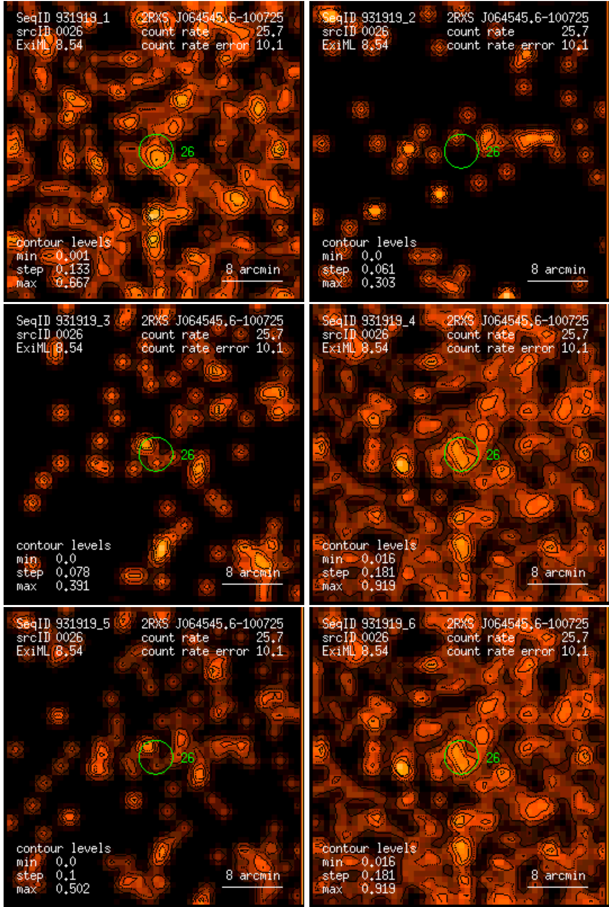
Figure 26: RASS 931919: detection 0026: band rate images, Gaussian filter: (1) PSPC channels 11 – 41, (2) 52 – 90, (3) 91 – 201, (4) 11 – 235, (5) 52 – 201, (6) 11 – 201. Broad band rates in counts/ks. Band rate contour levels in counts/ks/arcmin 2 .
