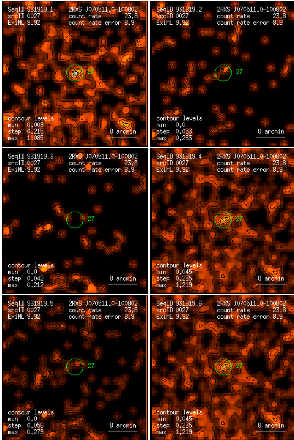
Figure 27: RASS 931919: detection 0027: band rate images, Gaussian filter: (1) PSPC channels 11 – 41, (2) 52 – 90, (3) 91 – 201, (4) 11 – 235, (5) 52 – 201, (6) 11 – 201. Broad band rates in counts/ks. Band rate contour levels in counts/ks/arcmin 2 .
