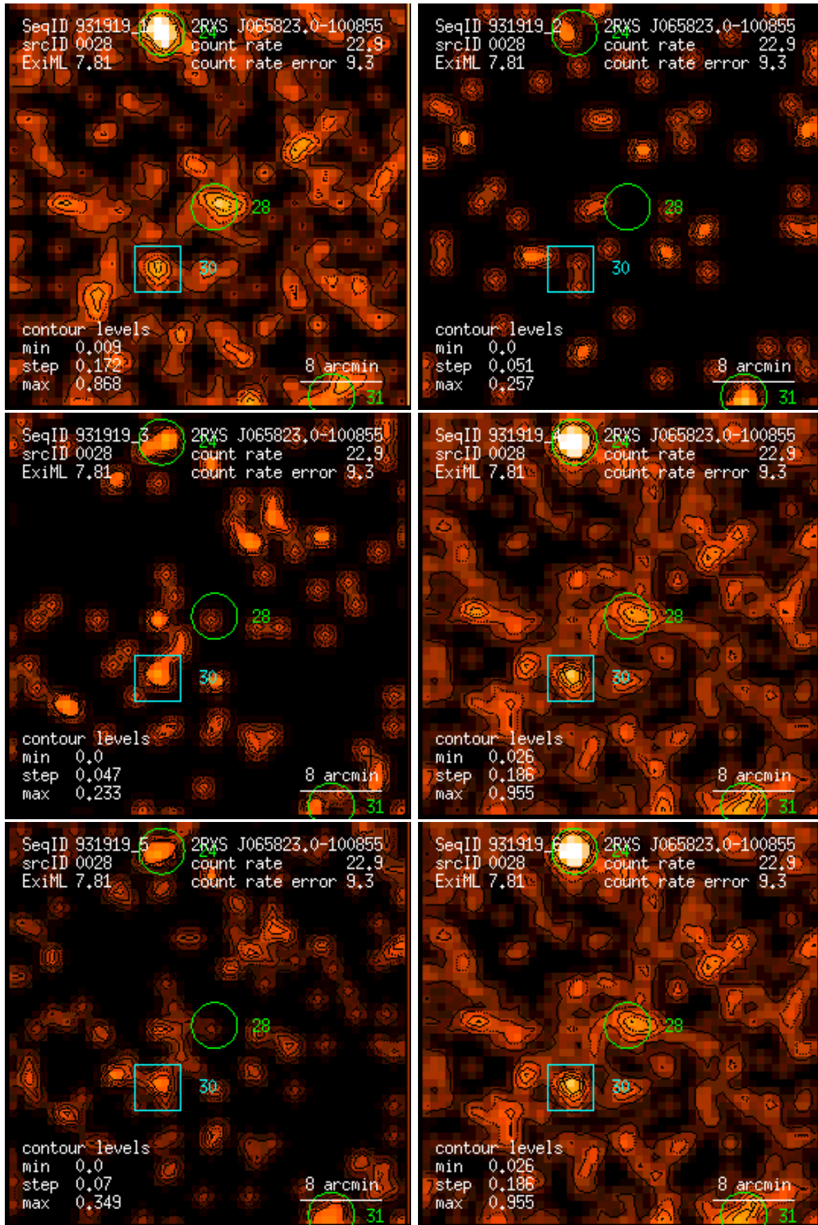
Figure 28: RASS 931919: detection 0028: band rate images, Gaussian filter: (1) PSPC channels 11 – 41, (2) 52 – 90, (3) 91 – 201, (4) 11 – 235, (5) 52 – 201, (6) 11 – 201. Broad band rates in counts/ks. Band rate contour levels in counts/ks/arcmin 2 .
