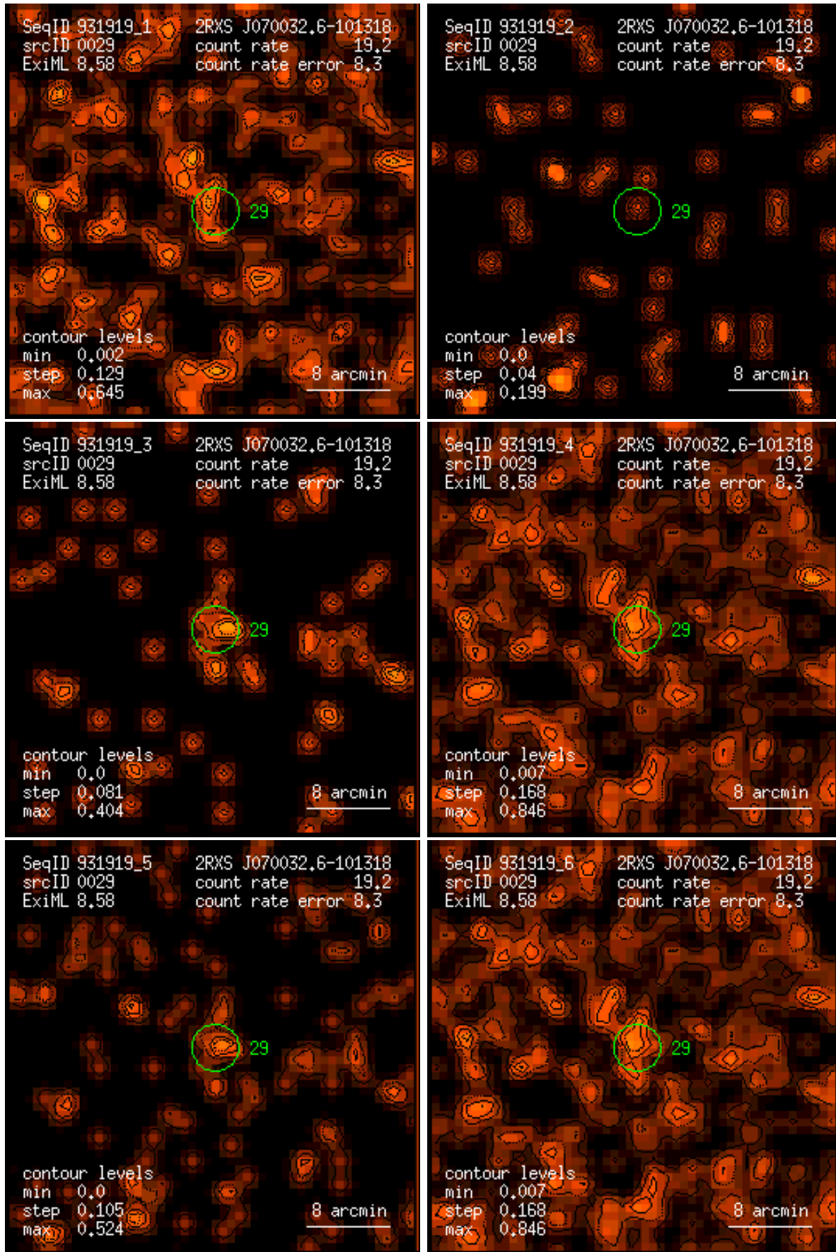
Figure 29: RASS 931919: detection 0029: band rate images, Gaussian filter: (1) PSPC channels 11 – 41, (2) 52 – 90, (3) 91 – 201, (4) 11 – 235, (5) 52 – 201, (6) 11 – 201. Broad band rates in counts/ks. Band rate contour levels in counts/ks/arcmin 2 .
