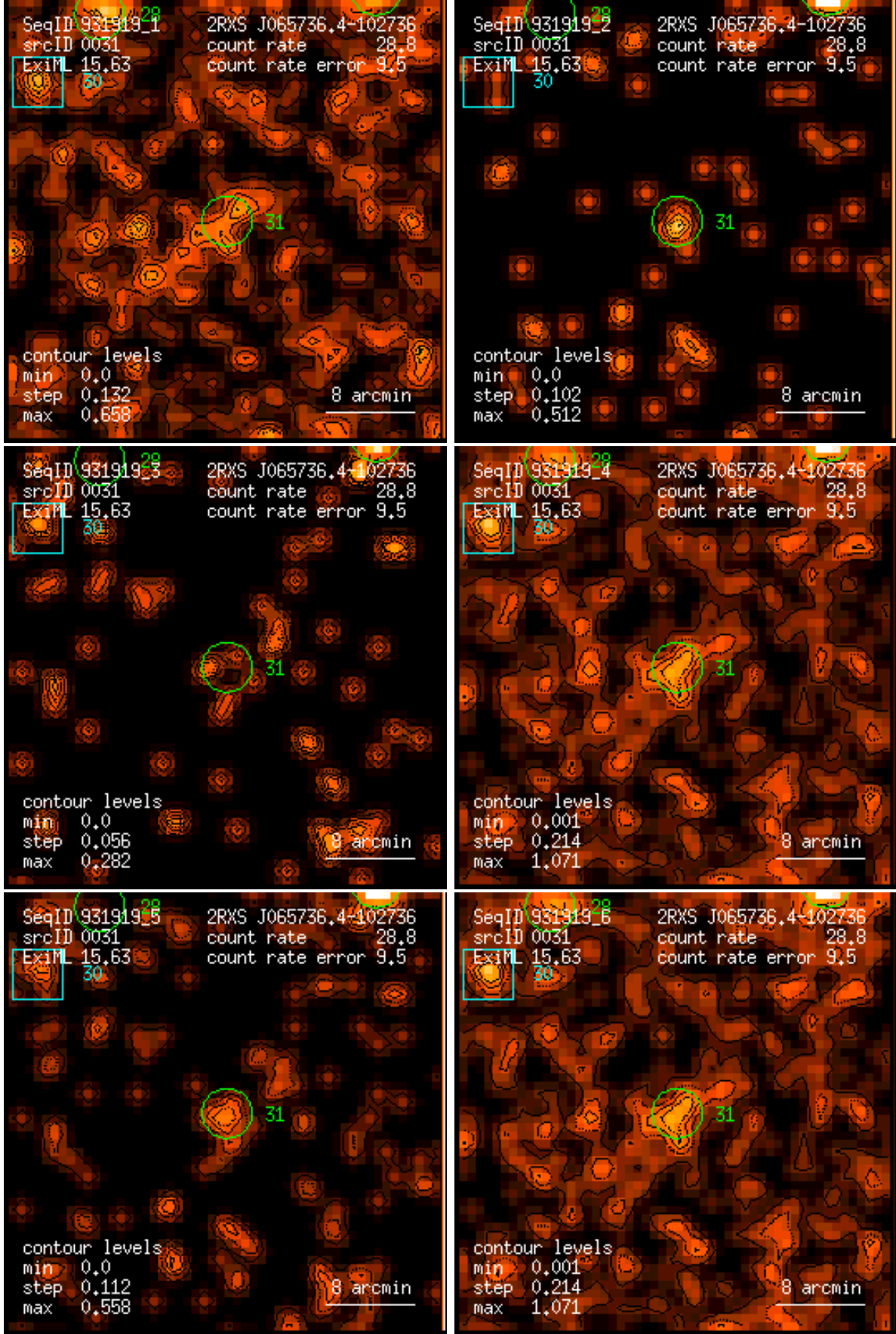
Figure 31: RASS 931919: detection 0031: band rate images, Gaussian filter: (1) PSPC channels 11 – 41, (2) 52 – 90, (3) 91 – 201, (4) 11 – 235, (5) 52 – 201, (6) 11 – 201. Broad band rates in counts/ks. Band rate contour levels in counts/ks/arcmin 2 .
