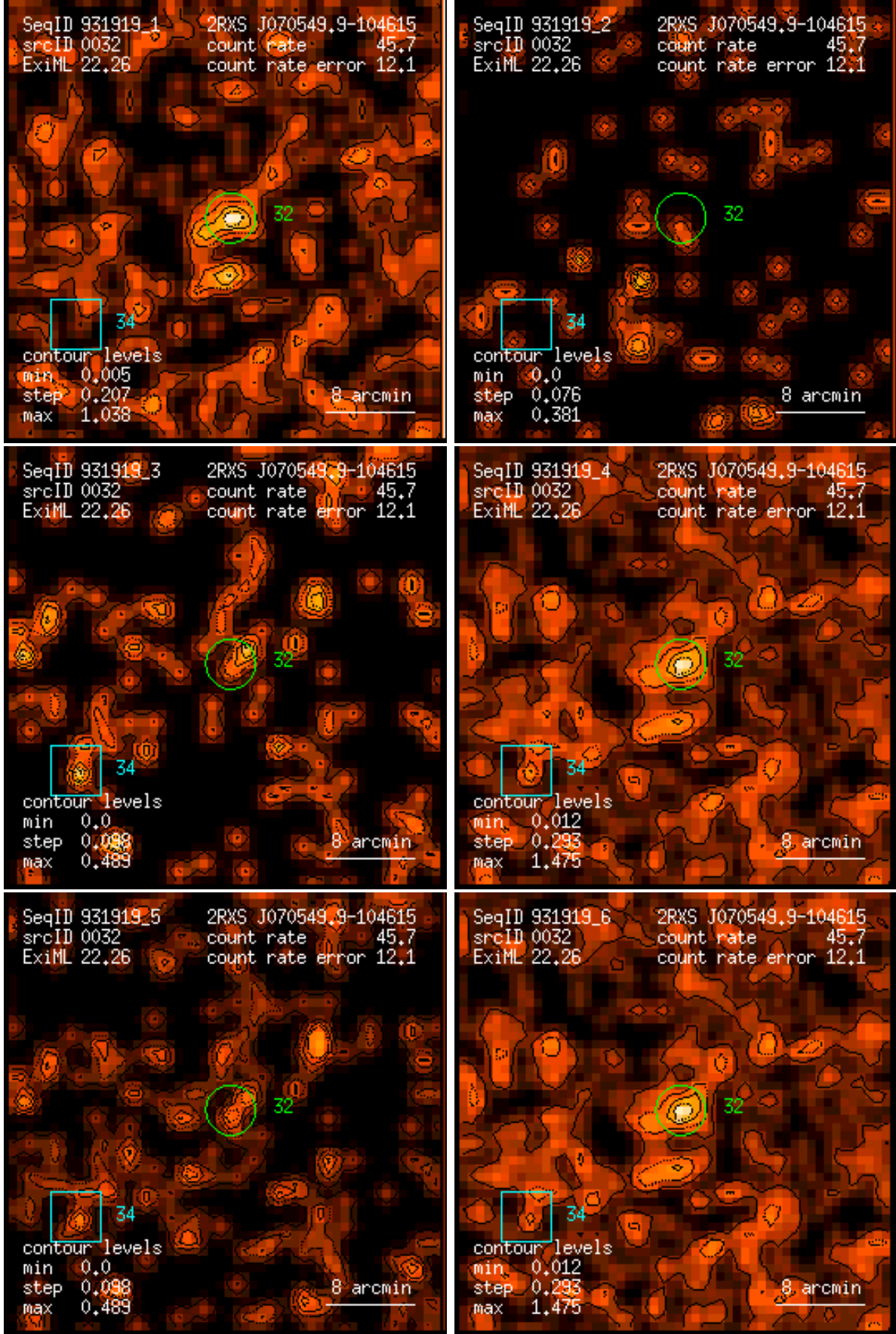
Figure 32: RASS 931919: detection 0032: band rate images, Gaussian filter: (1) PSPC channels 11 – 41, (2) 52 – 90, (3) 91 – 201, (4) 11 – 235, (5) 52 – 201, (6) 11 – 201. Broad band rates in counts/ks. Band rate contour levels in counts/ks/arcmin 2 .
