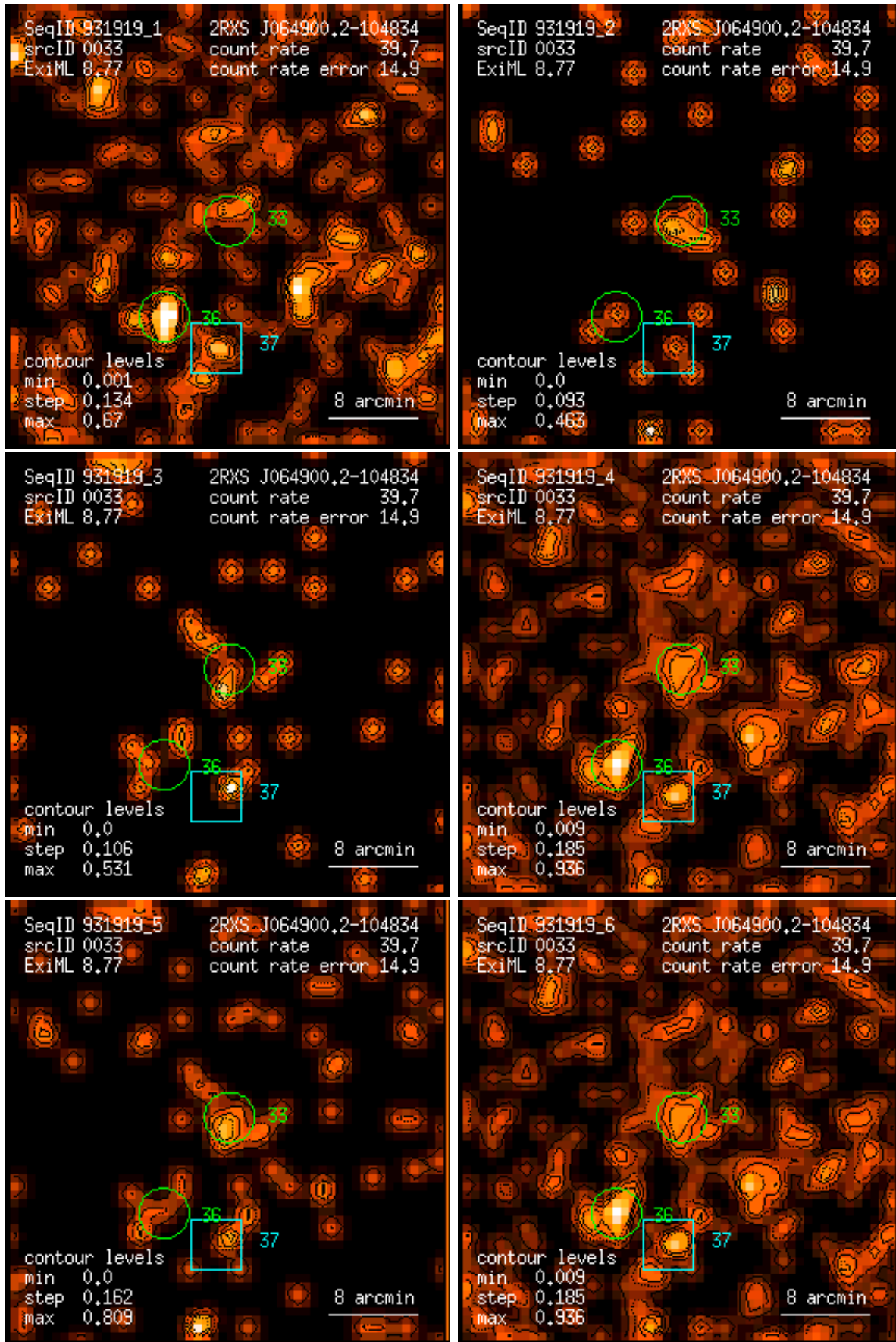
Figure 33: RASS 931919: detection 0033: band rate images, Gaussian filter: (1) PSPC channels 11 – 41, (2) 52 – 90, (3) 91 – 201, (4) 11 – 235, (5) 52 – 201, (6) 11 – 201. Broad band rates in counts/ks. Band rate contour levels in counts/ks/arcmin 2 .
