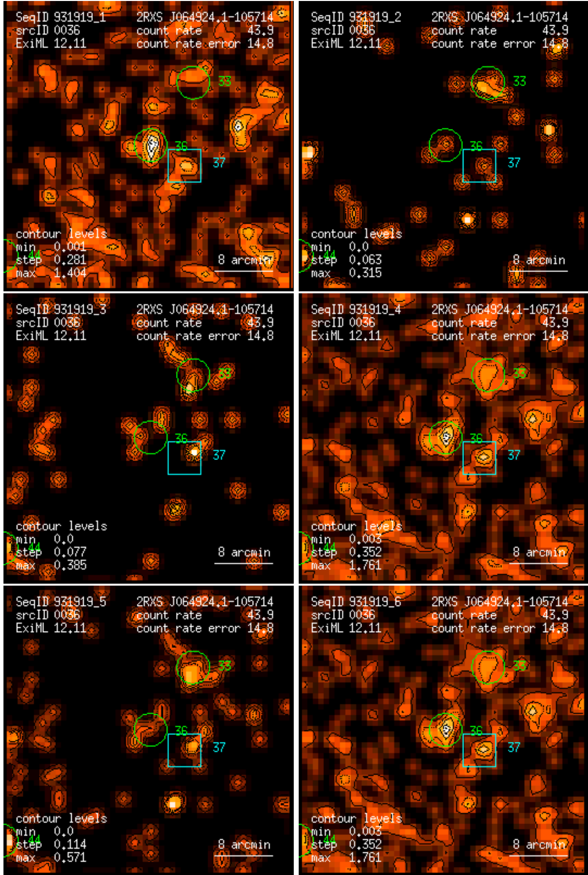
Figure 36: RASS 931919: detection 0036: band rate images, Gaussian filter: (1) PSPC channels 11 – 41, (2) 52 – 90, (3) 91 – 201, (4) 11 – 235, (5) 52 – 201, (6) 11 – 201. Broad band rates in counts/ks. Band rate contour levels in counts/ks/arcmin 2 .
