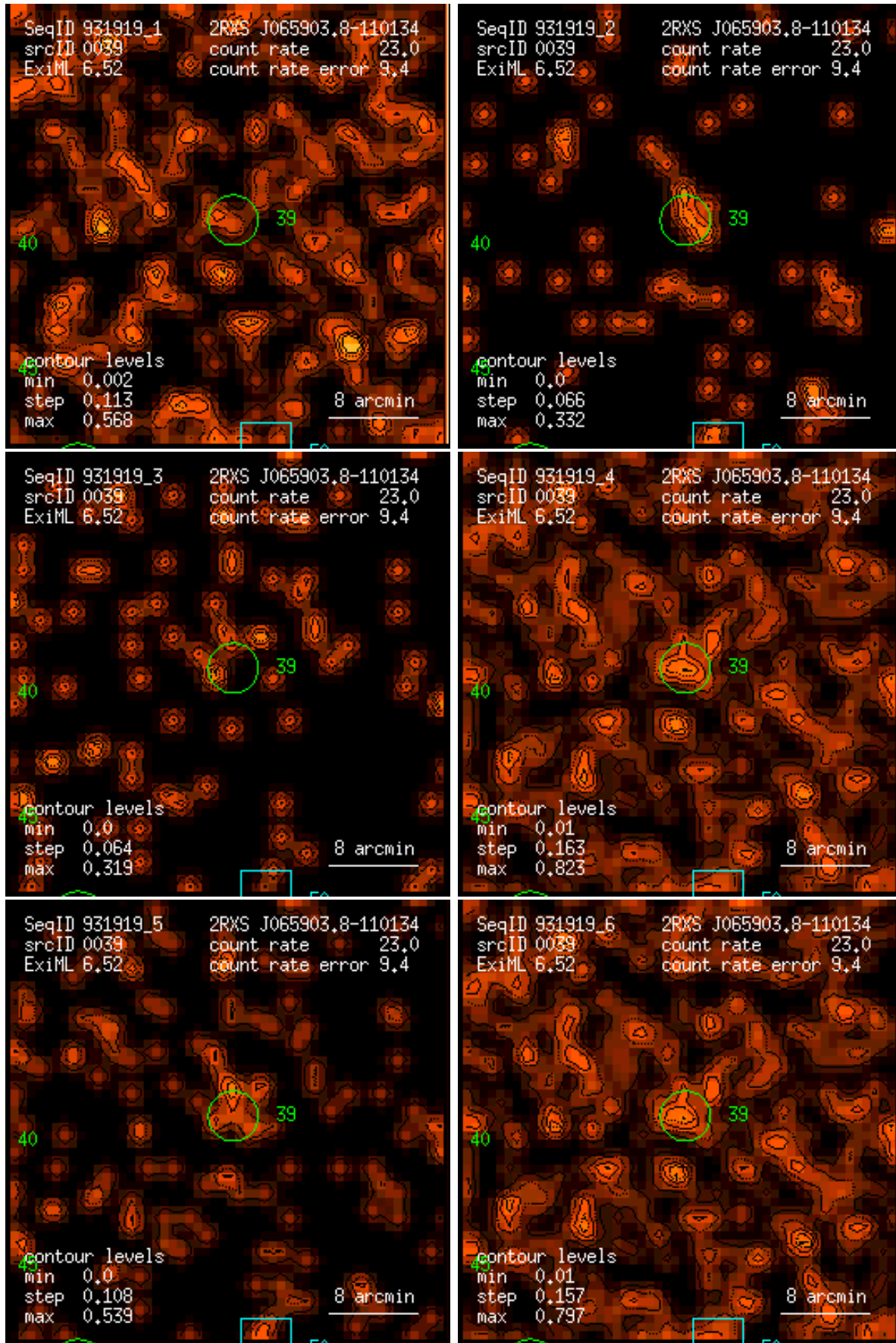
Figure 39: RASS 931919: detection 0039: band rate images, Gaussian filter: (1) PSPC channels 11 – 41, (2) 52 – 90, (3) 91 – 201, (4) 11 – 235, (5) 52 – 201, (6) 11 – 201. Broad band rates in counts/ks. Band rate contour levels in counts/ks/arcmin 2 .
