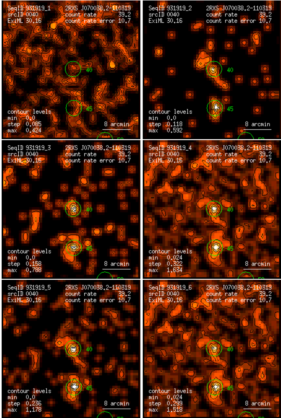
Figure 40: RASS 931919: detection 0040: band rate images, Gaussian filter: (1) PSPC channels 11 – 41, (2) 52 – 90, (3) 91 – 201, (4) 11 – 235, (5) 52 – 201, (6) 11 – 201. Broad band rates in counts/ks. Band rate contour levels in counts/ks/arcmin 2 .
