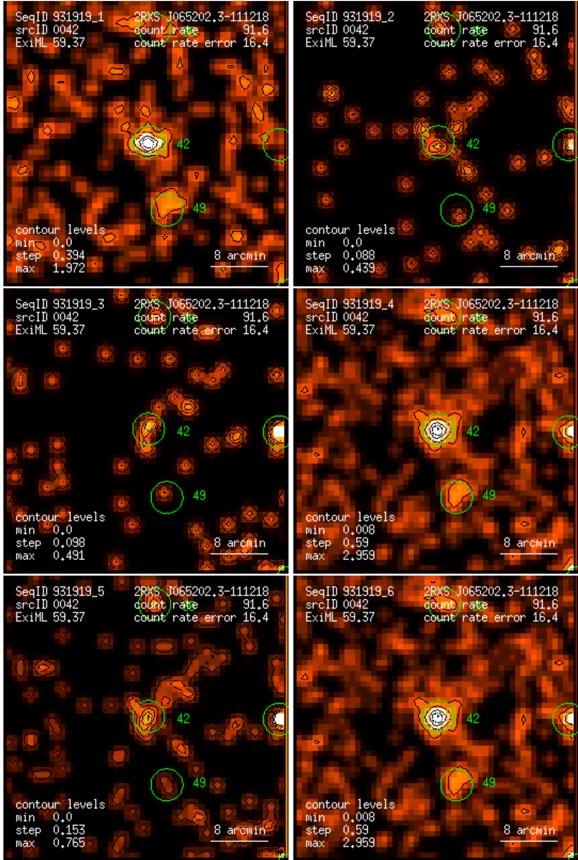
Figure 42: RASS 931919: detection 0042: band rate images, Gaussian filter: (1) PSPC channels 11 – 41, (2) 52 – 90, (3) 91 – 201, (4) 11 – 235, (5) 52 – 201, (6) 11 – 201. Broad band rates in counts/ks. Band rate contour levels in counts/ks/arcmin 2 .
