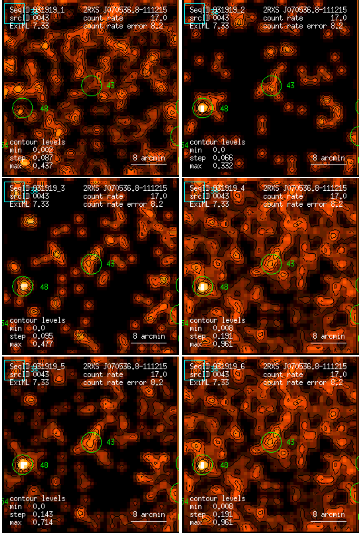
Figure 43: RASS 931919: detection 0043: band rate images, Gaussian filter: (1) PSPC channels 11 – 41, (2) 52 – 90, (3) 91 – 201, (4) 11 – 235, (5) 52 – 201, (6) 11 – 201. Broad band rates in counts/ks. Band rate contour levels in counts/ks/arcmin 2 .
