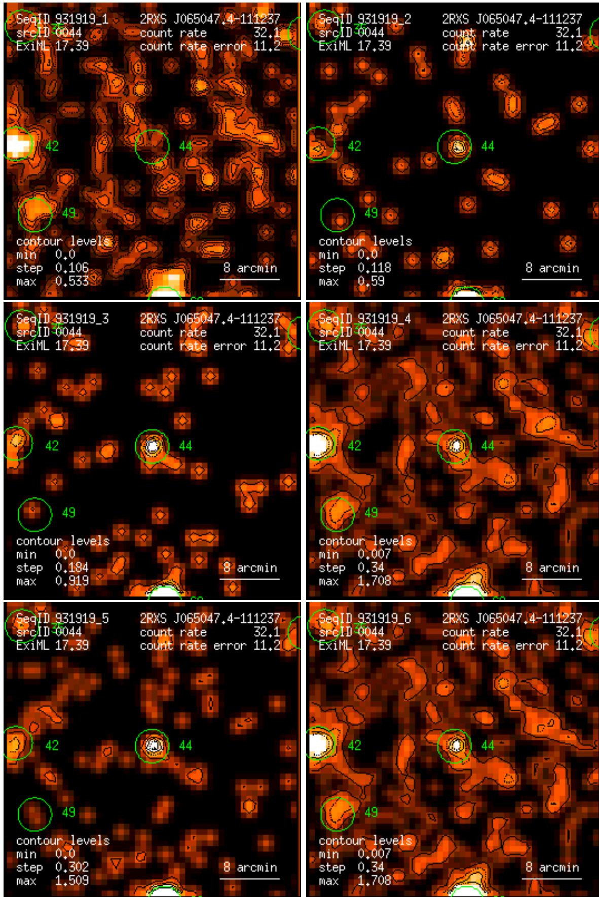
Figure 44: RASS 931919: detection 0044: band rate images, Gaussian filter: (1) PSPC channels 11 – 41, (2) 52 – 90, (3) 91 – 201, (4) 11 – 235, (5) 52 – 201, (6) 11 – 201. Broad band rates in counts/ks. Band rate contour levels in counts/ks/arcmin 2 .
