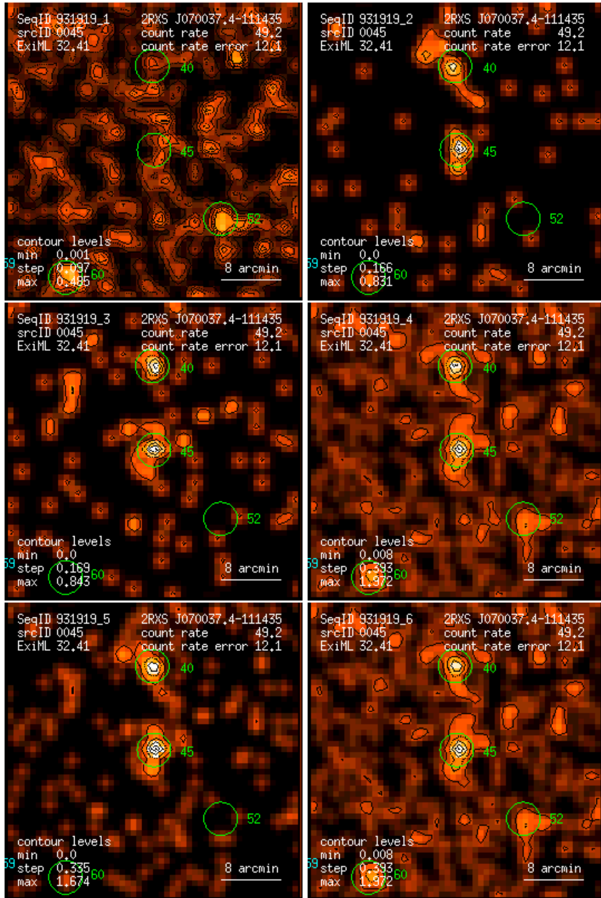
Figure 45: RASS 931919: detection 0045: band rate images, Gaussian filter: (1) PSPC channels 11 – 41, (2) 52 – 90, (3) 91 – 201, (4) 11 – 235, (5) 52 – 201, (6) 11 – 201. Broad band rates in counts/ks. Band rate contour levels in counts/ks/arcmin 2 .
