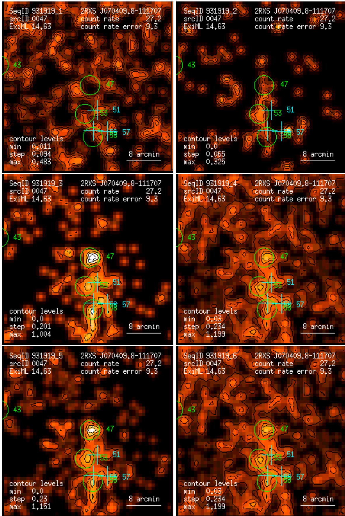
Figure 47: RASS 931919: detection 0047: band rate images, Gaussian filter: (1) PSPC channels 11 – 41, (2) 52 – 90, (3) 91 – 201, (4) 11 – 235, (5) 52 – 201, (6) 11 – 201. Broad band rates in counts/ks. Band rate contour levels in counts/ks/arcmin 2 .
