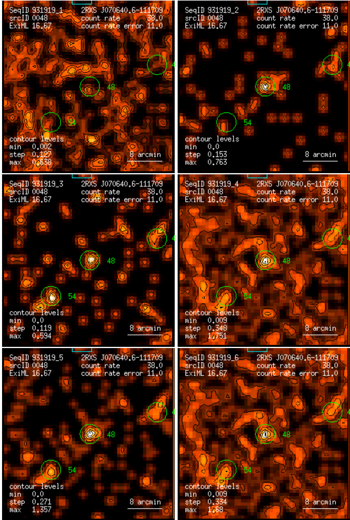
Figure 48: RASS 931919: detection 0048: band rate images, Gaussian filter: (1) PSPC channels 11 – 41, (2) 52 – 90, (3) 91 – 201, (4) 11 – 235, (5) 52 – 201, (6) 11 – 201. Broad band rates in counts/ks. Band rate contour levels in counts/ks/arcmin 2 .
