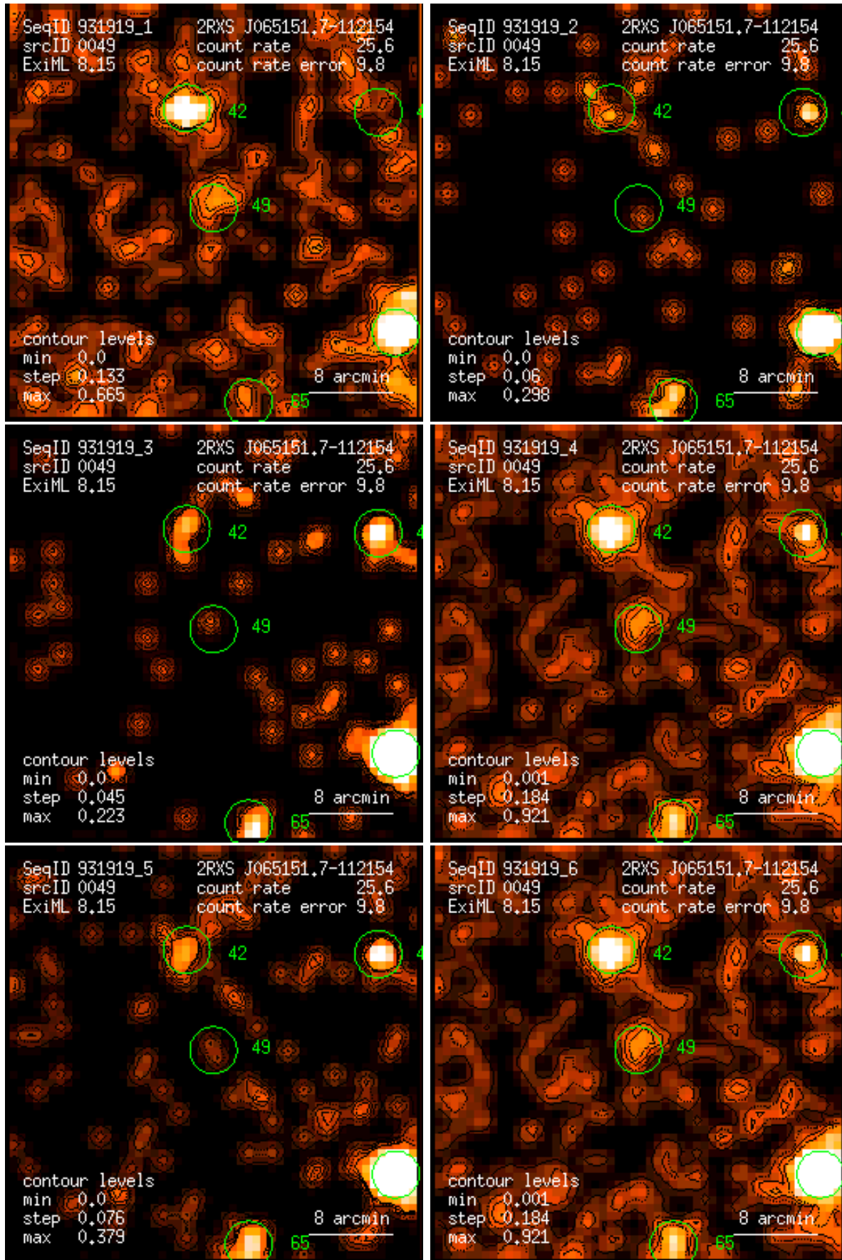
Figure 49: RASS 931919: detection 0049: band rate images, Gaussian filter: (1) PSPC channels 11 – 41, (2) 52 – 90, (3) 91 – 201, (4) 11 – 235, (5) 52 – 201, (6) 11 – 201. Broad band rates in counts/ks. Band rate contour levels in counts/ks/arcmin 2 .
