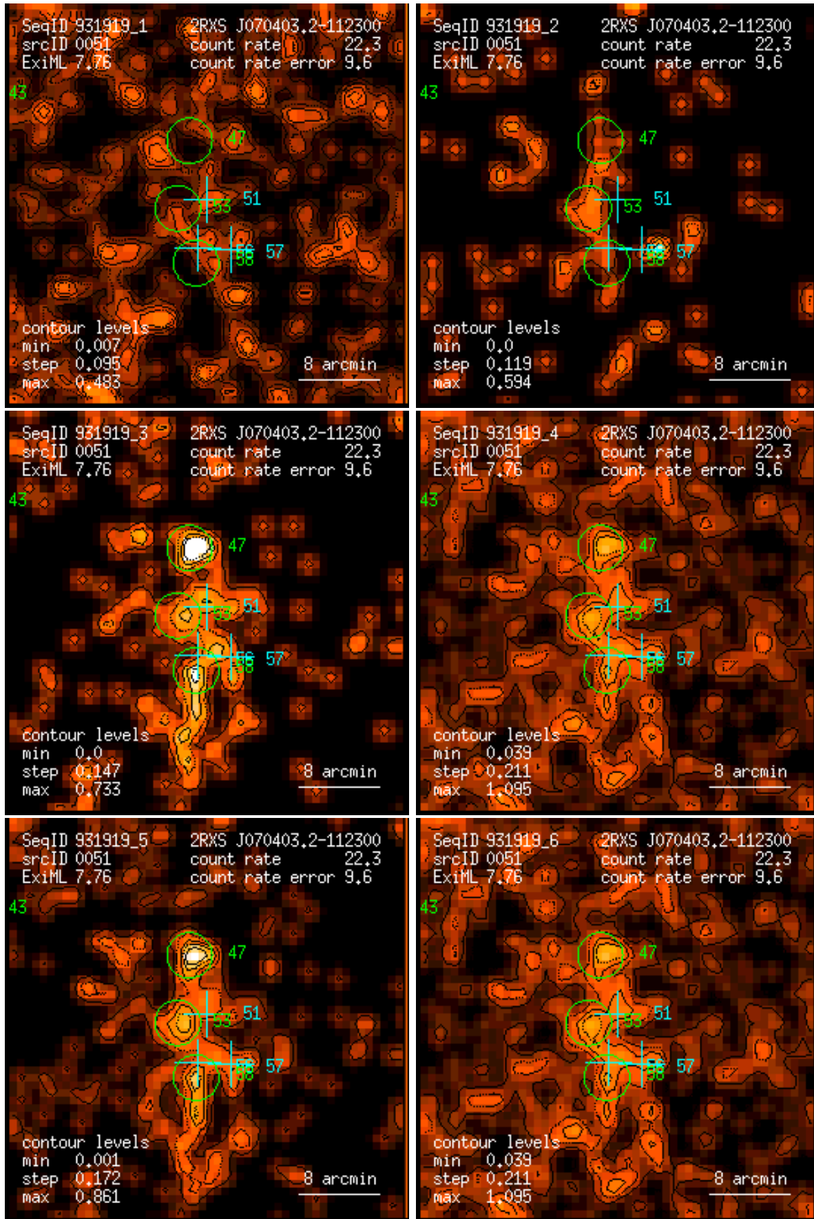
Figure 51: RASS 931919: detection 0051: band rate images, Gaussian filter: (1) PSPC channels 11 – 41, (2) 52 – 90, (3) 91 – 201, (4) 11 – 235, (5) 52 – 201, (6) 11 – 201. Broad band rates in counts/ks. Band rate contour levels in counts/ks/arcmin 2 .
