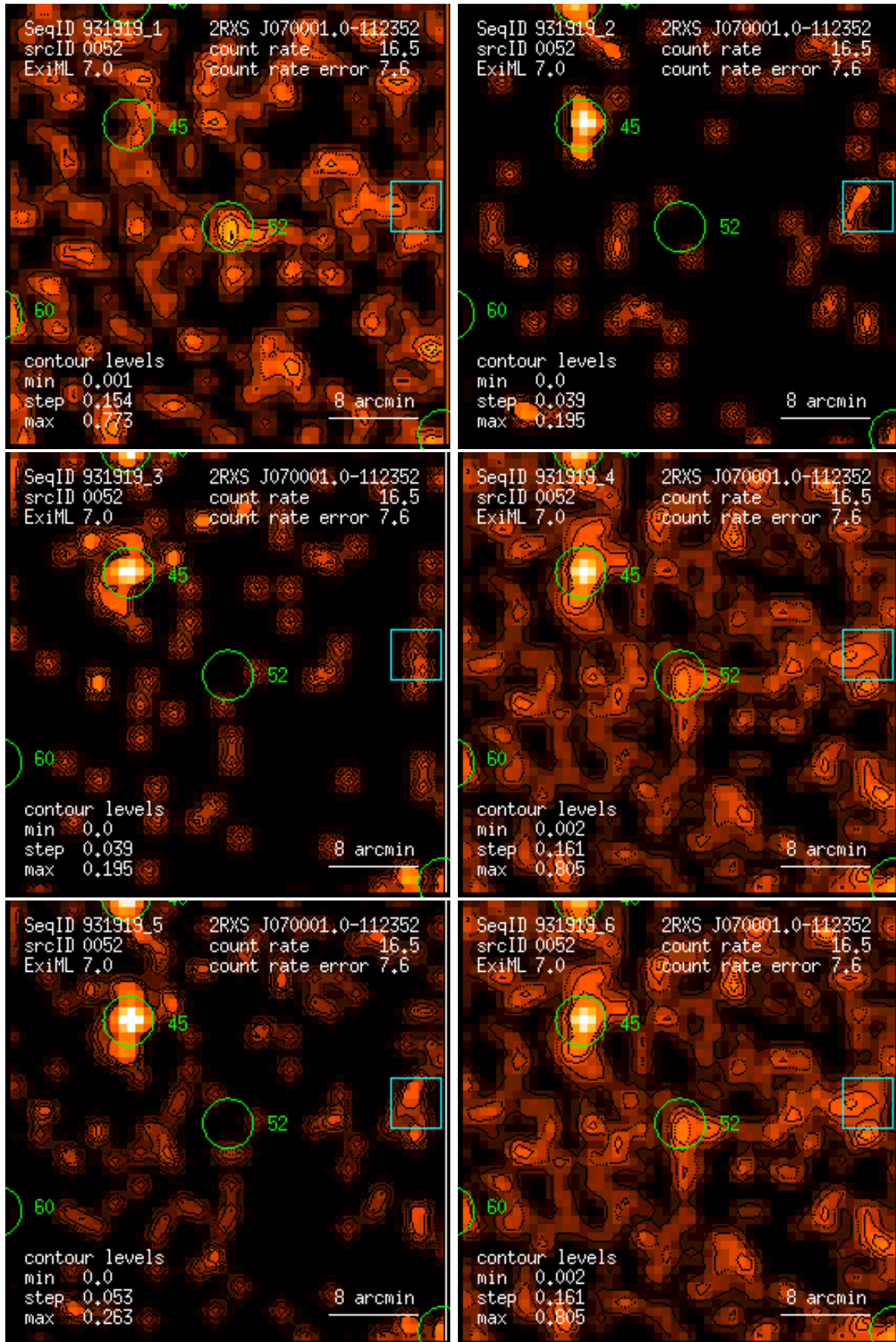
Figure 52: RASS 931919: detection 0052: band rate images, Gaussian filter: (1) PSPC channels 11 – 41, (2) 52 – 90, (3) 91 – 201, (4) 11 – 235, (5) 52 – 201, (6) 11 – 201. Broad band rates in counts/ks. Band rate contour levels in counts/ks/arcmin 2 .
