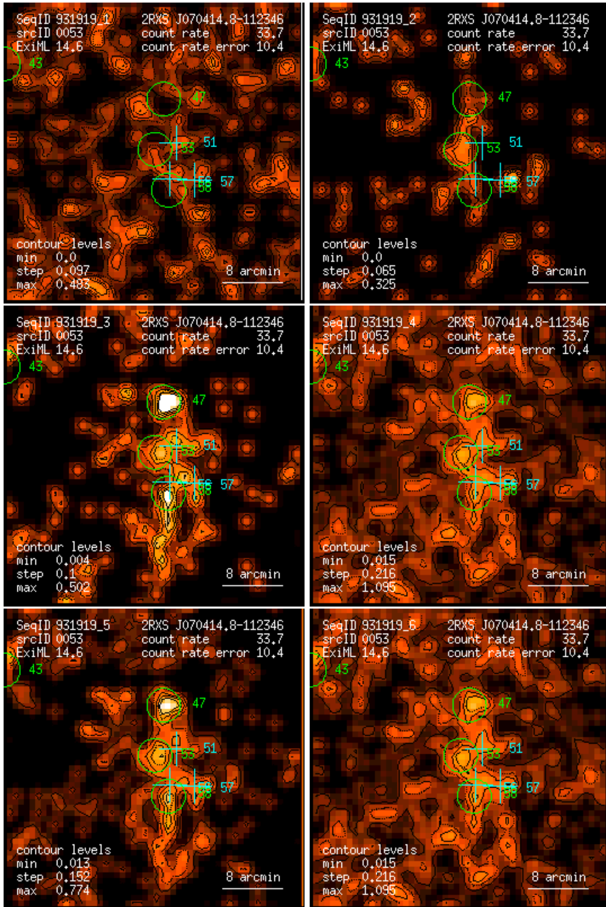
Figure 53: RASS 931919: detection 0053: band rate images, Gaussian filter: (1) PSPC channels 11 – 41, (2) 52 – 90, (3) 91 – 201, (4) 11 – 235, (5) 52 – 201, (6) 11 – 201. Broad band rates in counts/ks. Band rate contour levels in counts/ks/arcmin 2 .
