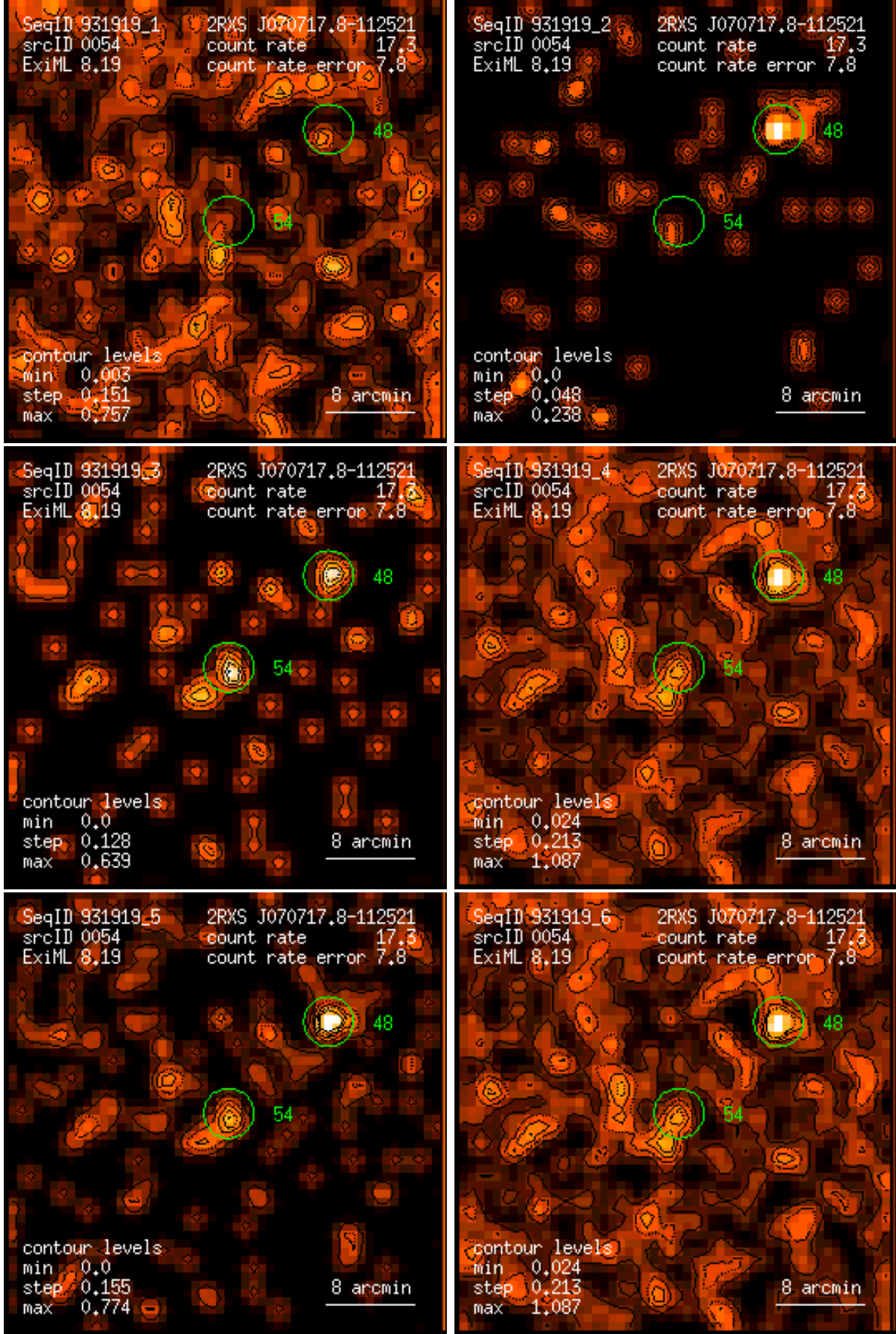
Figure 54: RASS 931919: detection 0054: band rate images, Gaussian filter: (1) PSPC channels 11 – 41, (2) 52 – 90, (3) 91 – 201, (4) 11 – 235, (5) 52 – 201, (6) 11 – 201. Broad band rates in counts/ks. Band rate contour levels in counts/ks/arcmin 2 .
