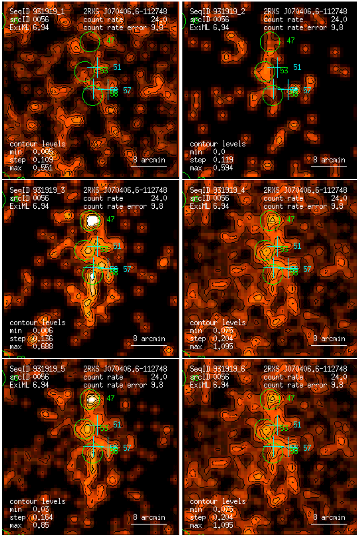
Figure 56: RASS 931919: detection 0056: band rate images, Gaussian filter: (1) PSPC channels 11 – 41, (2) 52 – 90, (3) 91 – 201, (4) 11 – 235, (5) 52 – 201, (6) 11 – 201. Broad band rates in counts/ks. Band rate contour levels in counts/ks/arcmin 2 .
