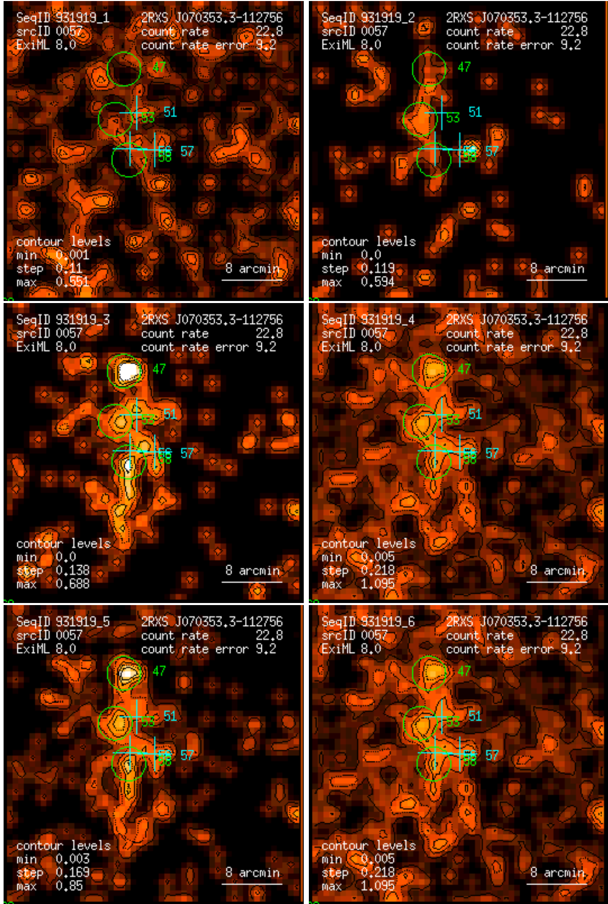
Figure 57: RASS 931919: detection 0057: band rate images, Gaussian filter: (1) PSPC channels 11 – 41, (2) 52 – 90, (3) 91 – 201, (4) 11 – 235, (5) 52 – 201, (6) 11 – 201. Broad band rates in counts/ks. Band rate contour levels in counts/ks/arcmin 2 .
