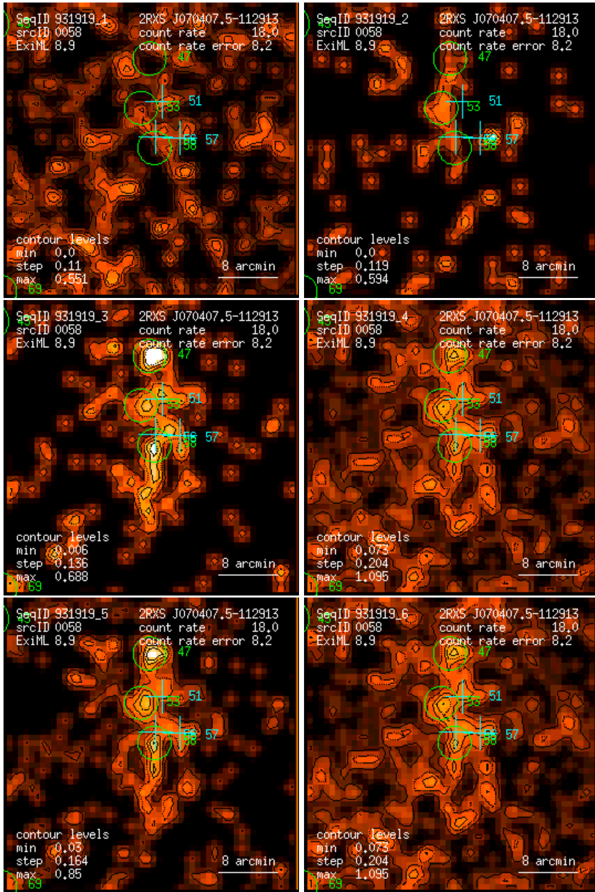
Figure 58: RASS 931919: detection 0058: band rate images, Gaussian filter: (1) PSPC channels 11 – 41, (2) 52 – 90, (3) 91 – 201, (4) 11 – 235, (5) 52 – 201, (6) 11 – 201. Broad band rates in counts/ks. Band rate contour levels in counts/ks/arcmin 2 .
