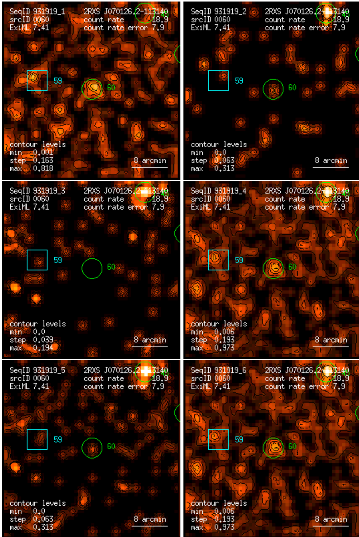
Figure 60: RASS 931919: detection 0060: band rate images, Gaussian filter: (1) PSPC channels 11 – 41, (2) 52 – 90, (3) 91 – 201, (4) 11 – 235, (5) 52 – 201, (6) 11 – 201. Broad band rates in counts/ks. Band rate contour levels in counts/ks/arcmin 2 .
