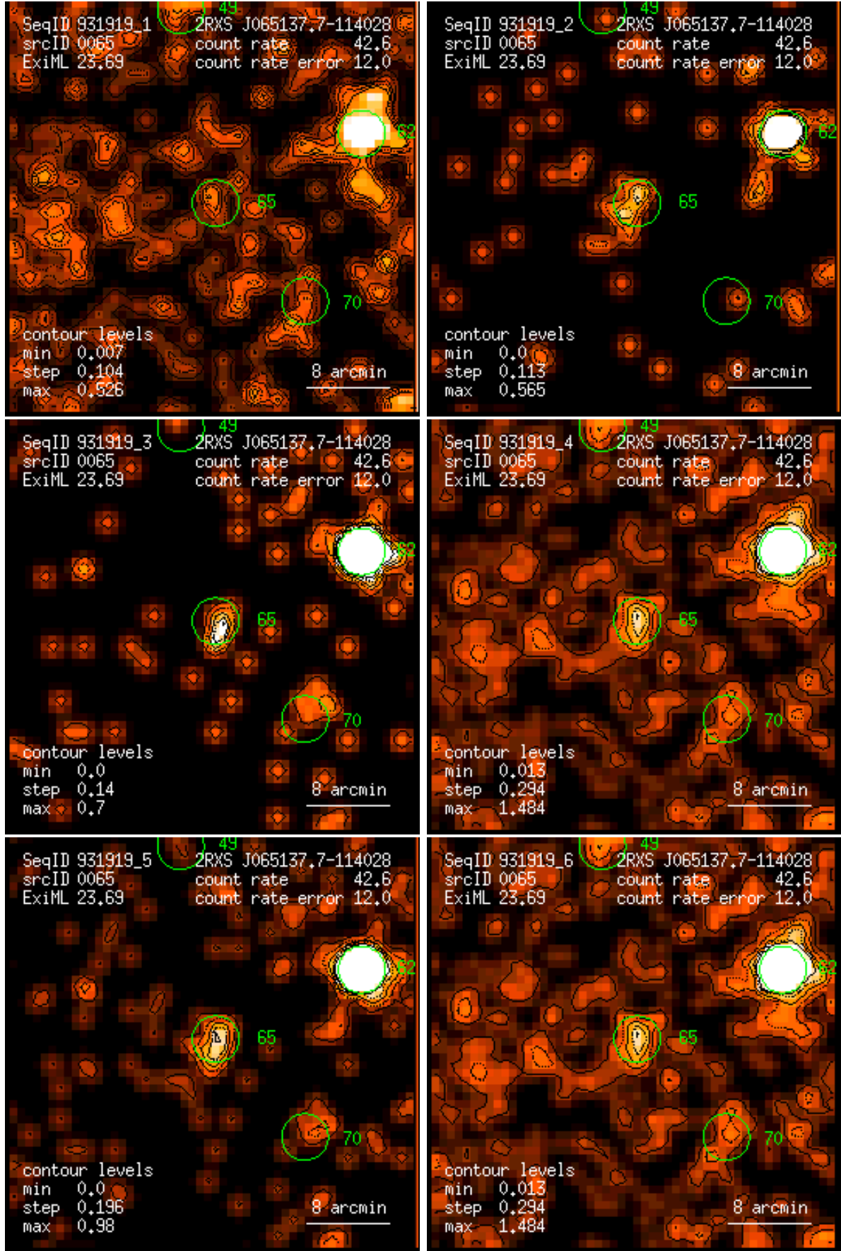
Figure 65: RASS 931919: detection 0065: band rate images, Gaussian filter: (1) PSPC channels 11 – 41, (2) 52 – 90, (3) 91 – 201, (4) 11 – 235, (5) 52 – 201, (6) 11 – 201. Broad band rates in counts/ks. Band rate contour levels in counts/ks/arcmin 2 .
