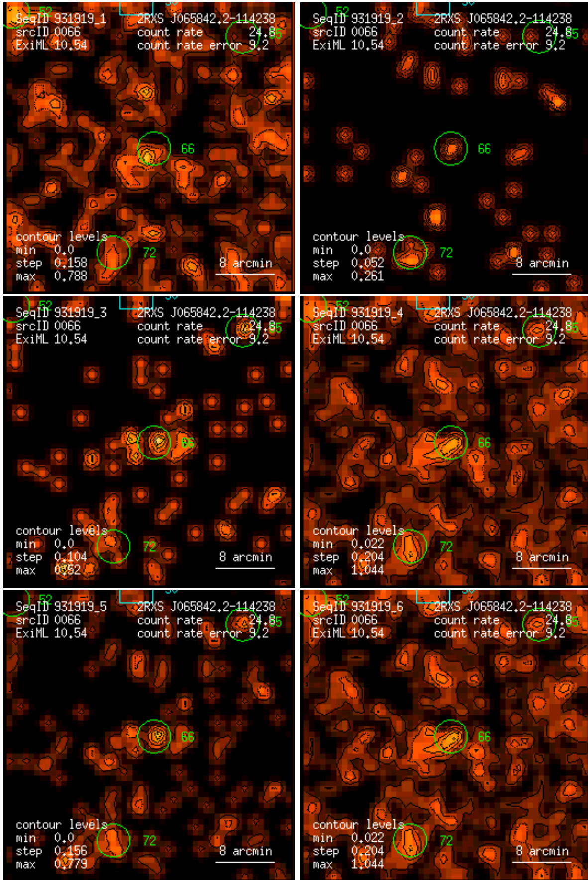
Figure 66: RASS 931919: detection 0066: band rate images, Gaussian filter: (1) PSPC channels 11 – 41, (2) 52 – 90, (3) 91 – 201, (4) 11 – 235, (5) 52 – 201, (6) 11 – 201. Broad band rates in counts/ks. Band rate contour levels in counts/ks/arcmin 2 .
