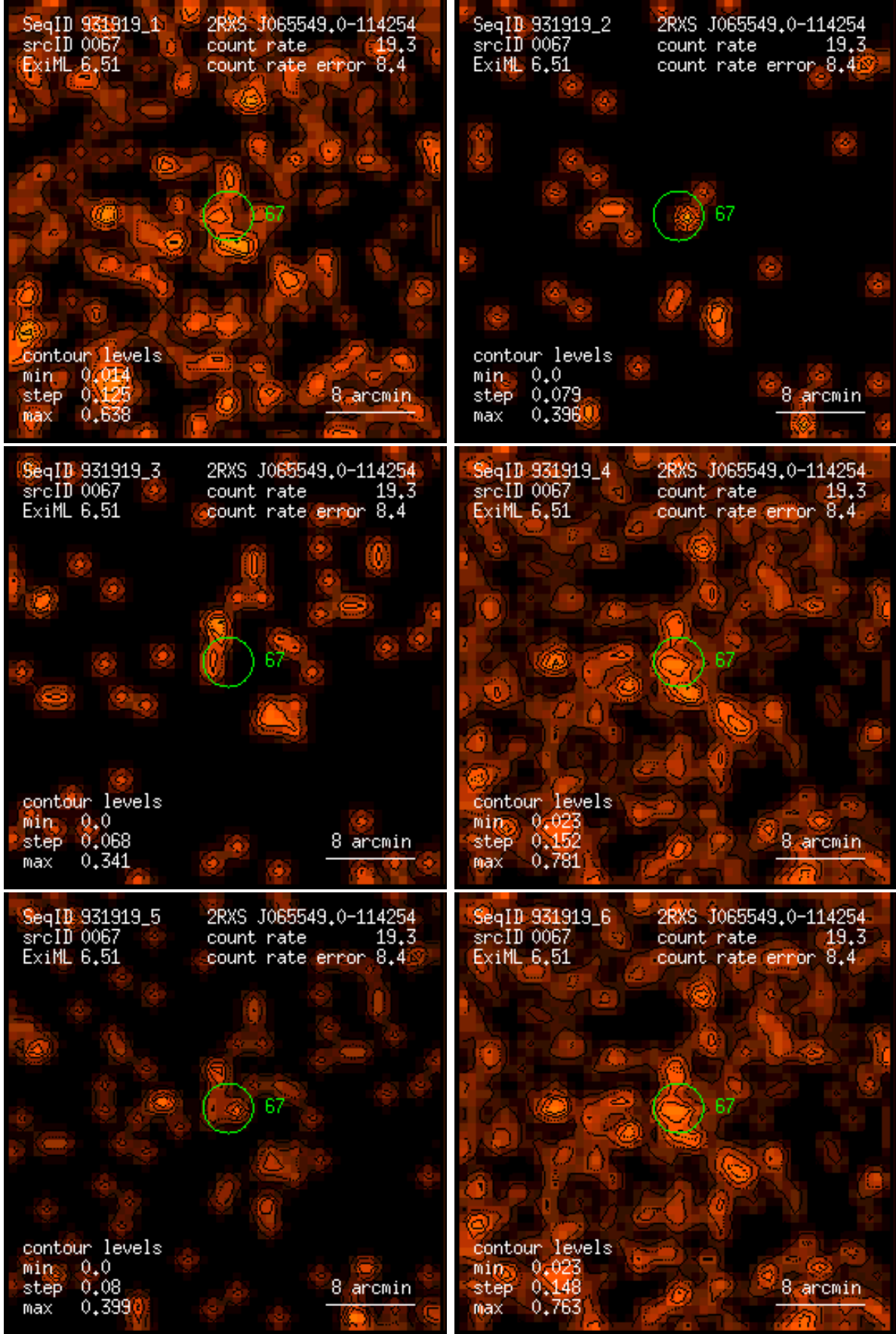
Figure 67: RASS 931919: detection 0067: band rate images, Gaussian filter: (1) PSPC channels 11 – 41, (2) 52 – 90, (3) 91 – 201, (4) 11 – 235, (5) 52 – 201, (6) 11 – 201. Broad band rates in counts/ks. Band rate contour levels in counts/ks/arcmin 2 .
