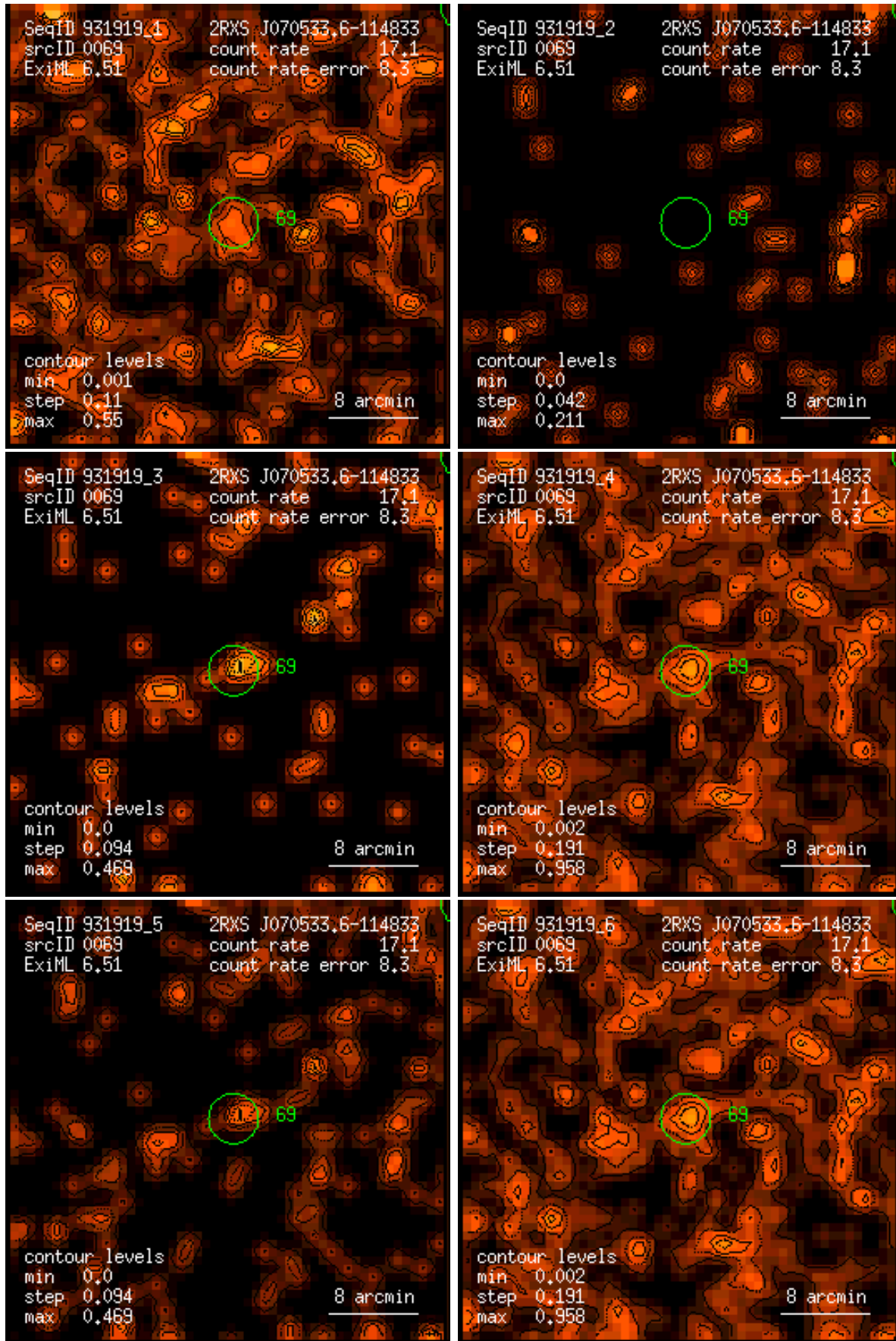
Figure 69: RASS 931919: detection 0069: band rate images, Gaussian filter: (1) PSPC channels 11 – 41, (2) 52 – 90, (3) 91 – 201, (4) 11 – 235, (5) 52 – 201, (6) 11 – 201. Broad band rates in counts/ks. Band rate contour levels in counts/ks/arcmin 2 .
