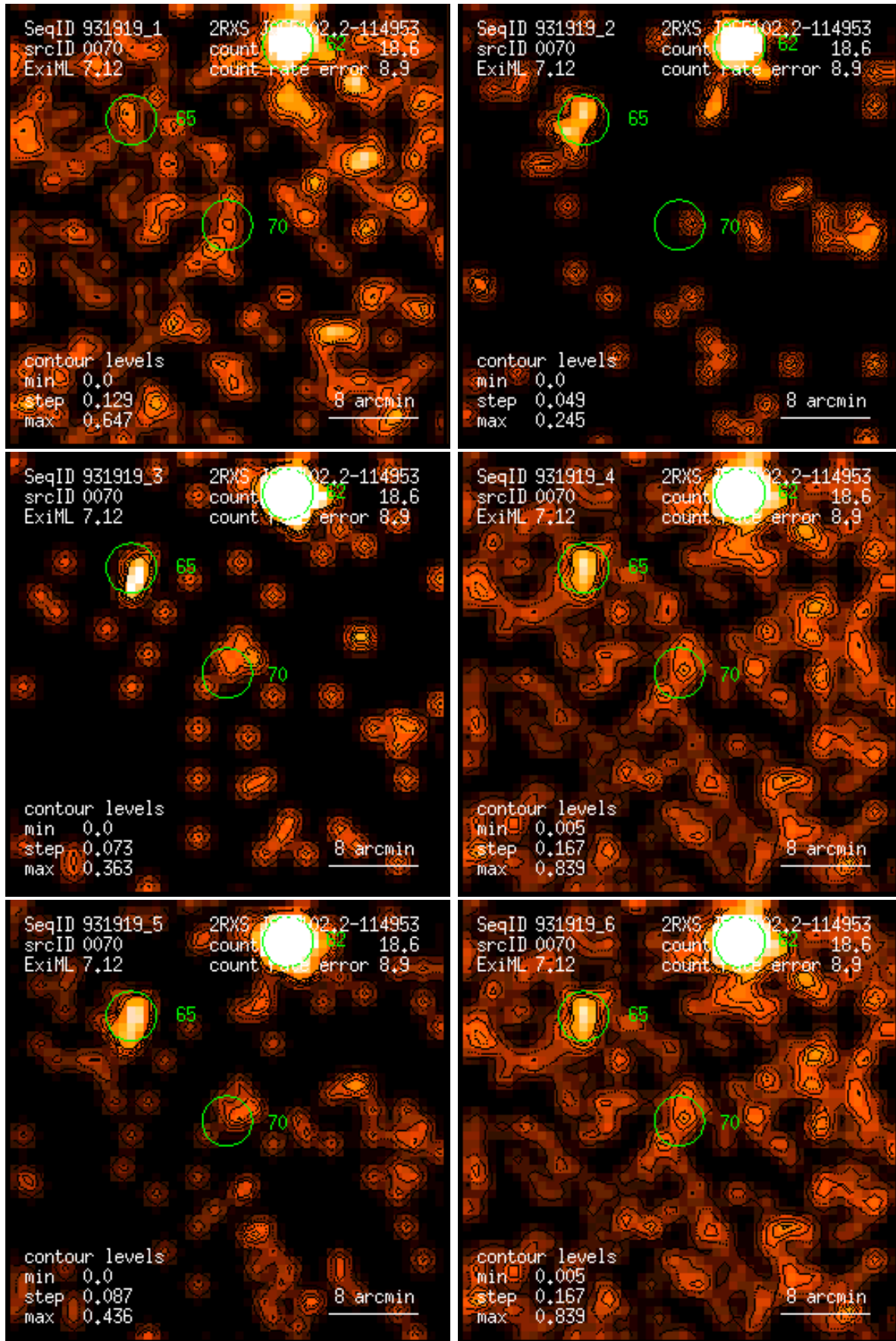
Figure 70: RASS 931919: detection 0070: band rate images, Gaussian filter: (1) PSPC channels 11 – 41, (2) 52 – 90, (3) 91 – 201, (4) 11 – 235, (5) 52 – 201, (6) 11 – 201. Broad band rates in counts/ks. Band rate contour levels in counts/ks/arcmin 2 .
