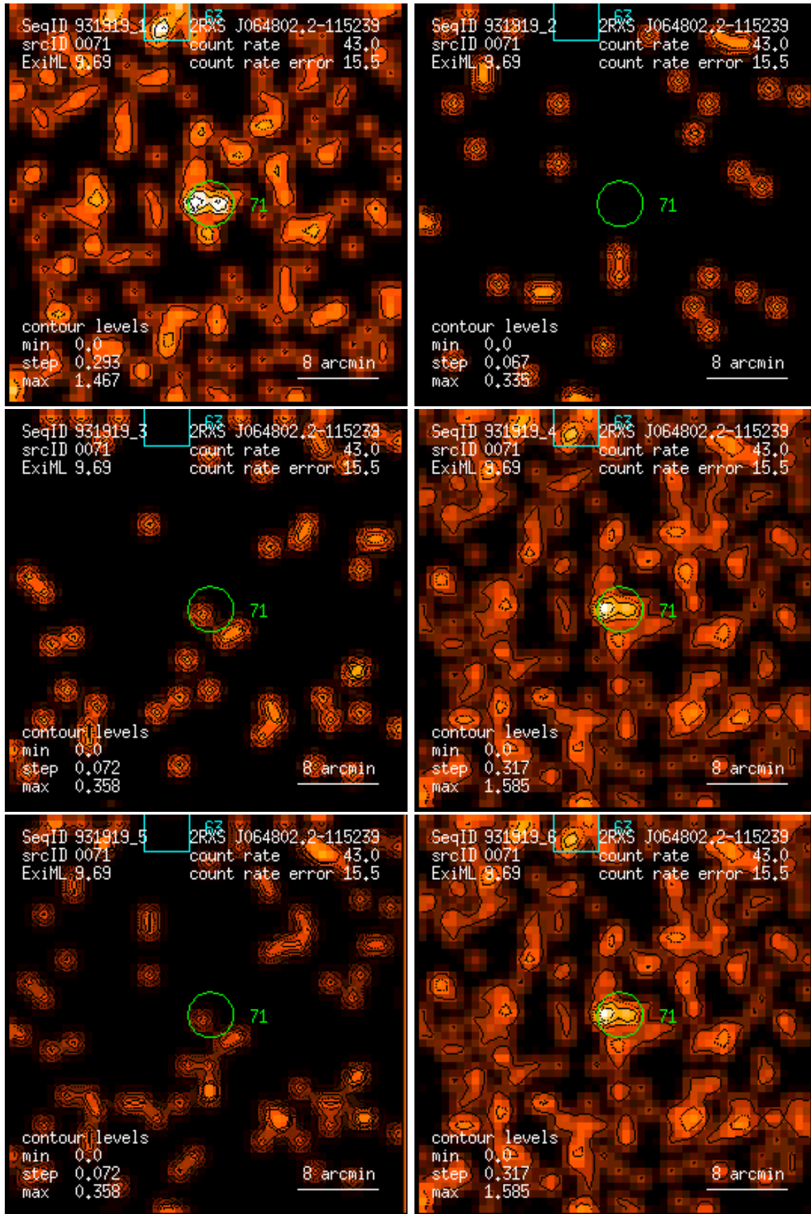
Figure 71: RASS 931919: detection 0071: band rate images, Gaussian filter: (1) PSPC channels 11 – 41, (2) 52 – 90, (3) 91 – 201, (4) 11 – 235, (5) 52 – 201, (6) 11 – 201. Broad band rates in counts/ks. Band rate contour levels in counts/ks/arcmin 2 .
