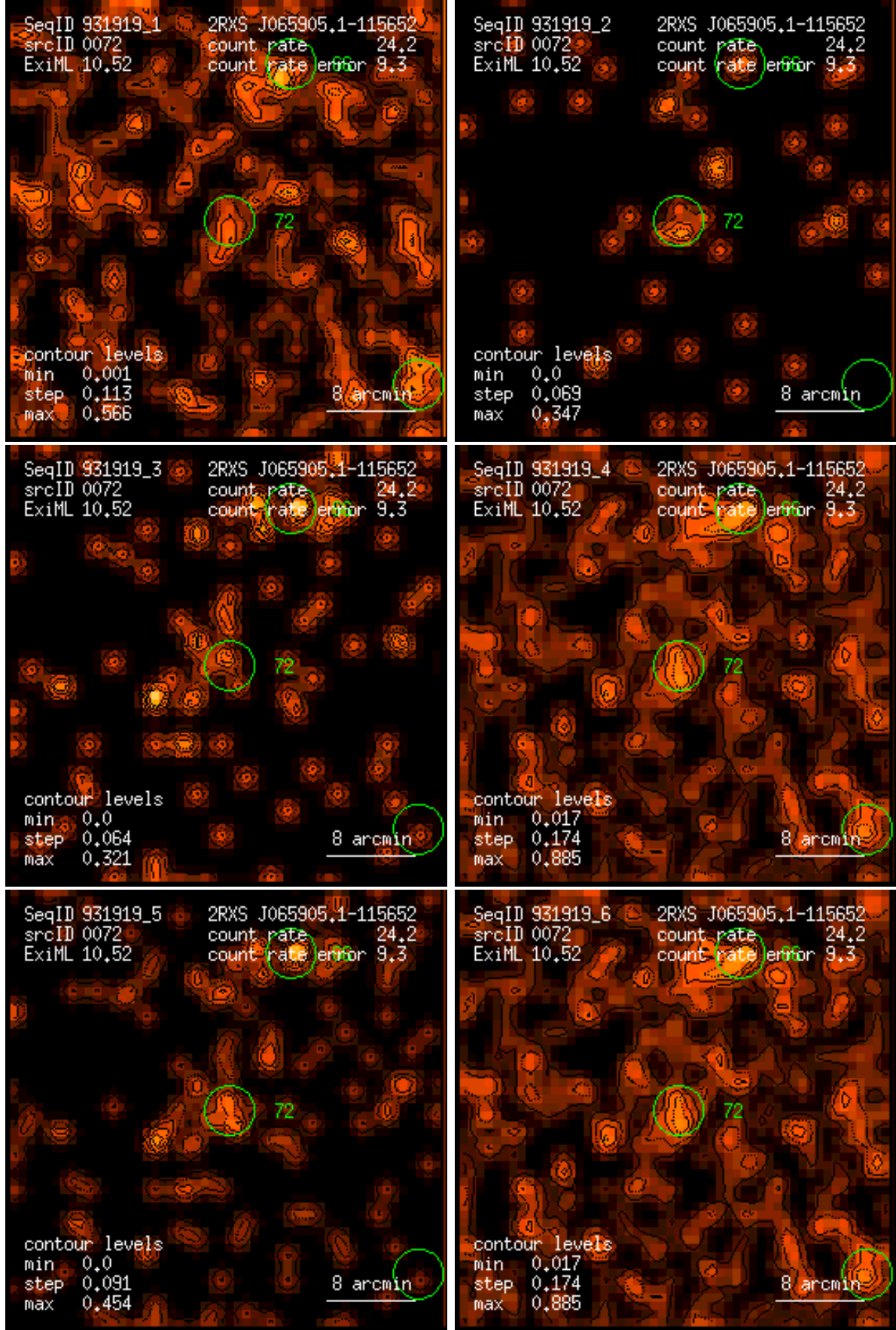
Figure 72: RASS 931919: detection 0072: band rate images, Gaussian filter: (1) PSPC channels 11 – 41, (2) 52 – 90, (3) 91 – 201, (4) 11 – 235, (5) 52 – 201, (6) 11 – 201. Broad band rates in counts/ks. Band rate contour levels in counts/ks/arcmin 2 .
