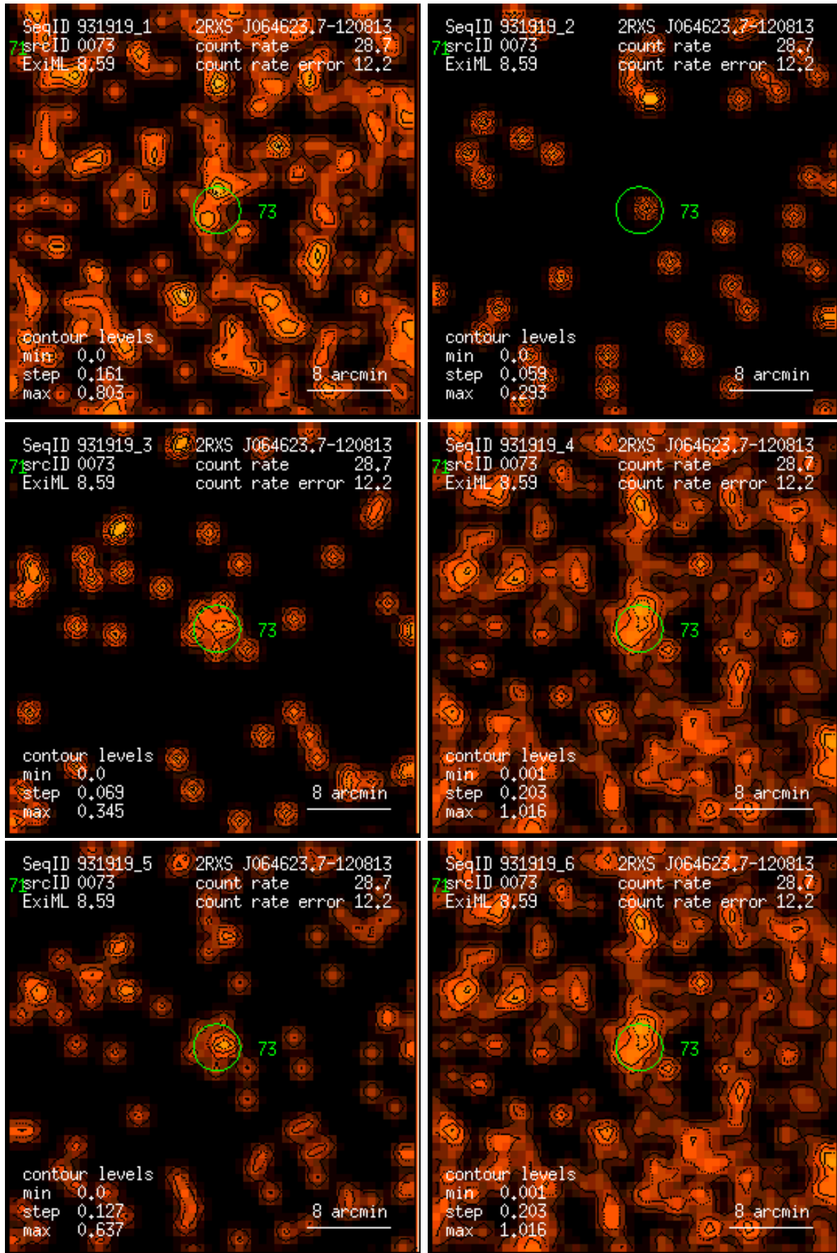
Figure 73: RASS 931919: detection 0073: band rate images, Gaussian filter: (1) PSPC channels 11 – 41, (2) 52 – 90, (3) 91 – 201, (4) 11 – 235, (5) 52 – 201, (6) 11 – 201. Broad band rates in counts/ks. Band rate contour levels in counts/ks/arcmin 2 .
