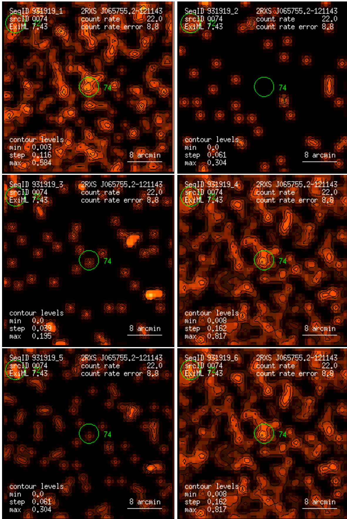
Figure 74: RASS 931919: detection 0074: band rate images, Gaussian filter: (1) PSPC channels 11 – 41, (2) 52 – 90, (3) 91 – 201, (4) 11 – 235, (5) 52 – 201, (6) 11 – 201. Broad band rates in counts/ks. Band rate contour levels in counts/ks/arcmin 2 .
