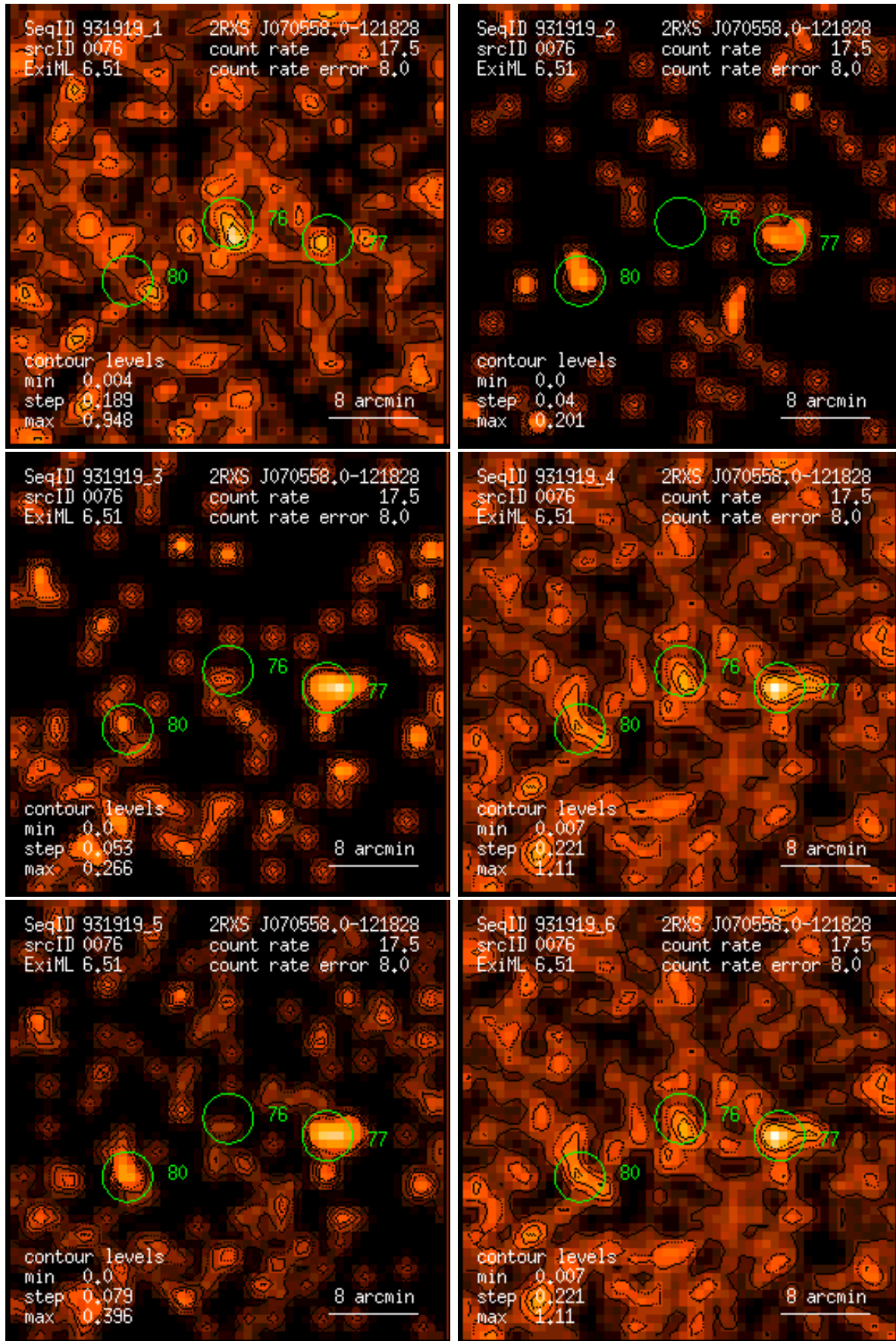
Figure 76: RASS 931919: detection 0076: band rate images, Gaussian filter: (1) PSPC channels 11 – 41, (2) 52 – 90, (3) 91 – 201, (4) 11 – 235, (5) 52 – 201, (6) 11 – 201. Broad band rates in counts/ks. Band rate contour levels in counts/ks/arcmin 2 .
