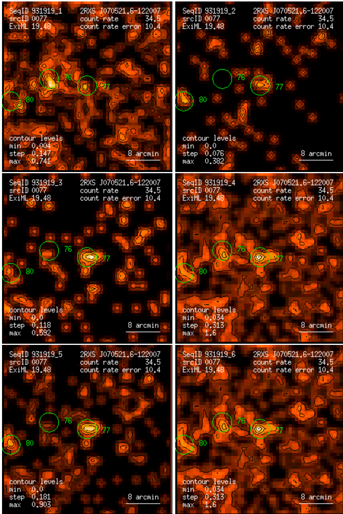
Figure 77: RASS 931919: detection 0077: band rate images, Gaussian filter: (1) PSPC channels 11 – 41, (2) 52 – 90, (3) 91 – 201, (4) 11 – 235, (5) 52 – 201, (6) 11 – 201. Broad band rates in counts/ks. Band rate contour levels in counts/ks/arcmin 2 .
