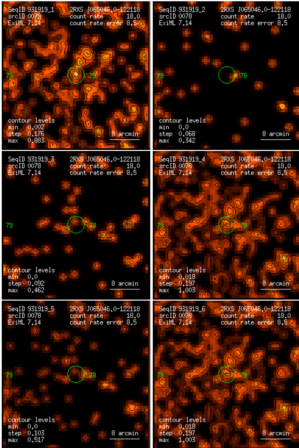
Figure 78: RASS 931919: detection 0078: band rate images, Gaussian filter: (1) PSPC channels 11 – 41, (2) 52 – 90, (3) 91 – 201, (4) 11 – 235, (5) 52 – 201, (6) 11 – 201. Broad band rates in counts/ks. Band rate contour levels in counts/ks/arcmin 2 .
