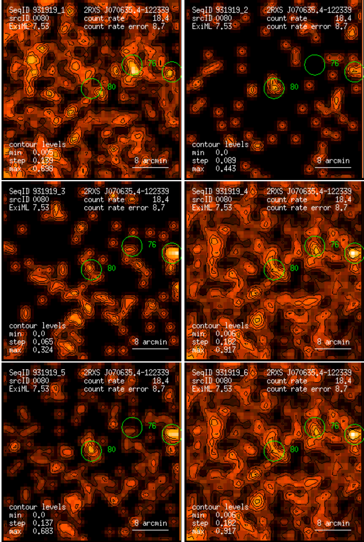
Figure 80: RASS 931919: detection 0080: band rate images, Gaussian filter: (1) PSPC channels 11 – 41, (2) 52 – 90, (3) 91 – 201, (4) 11 – 235, (5) 52 – 201, (6) 11 – 201. Broad band rates in counts/ks. Band rate contour levels in counts/ks/arcmin 2 .
