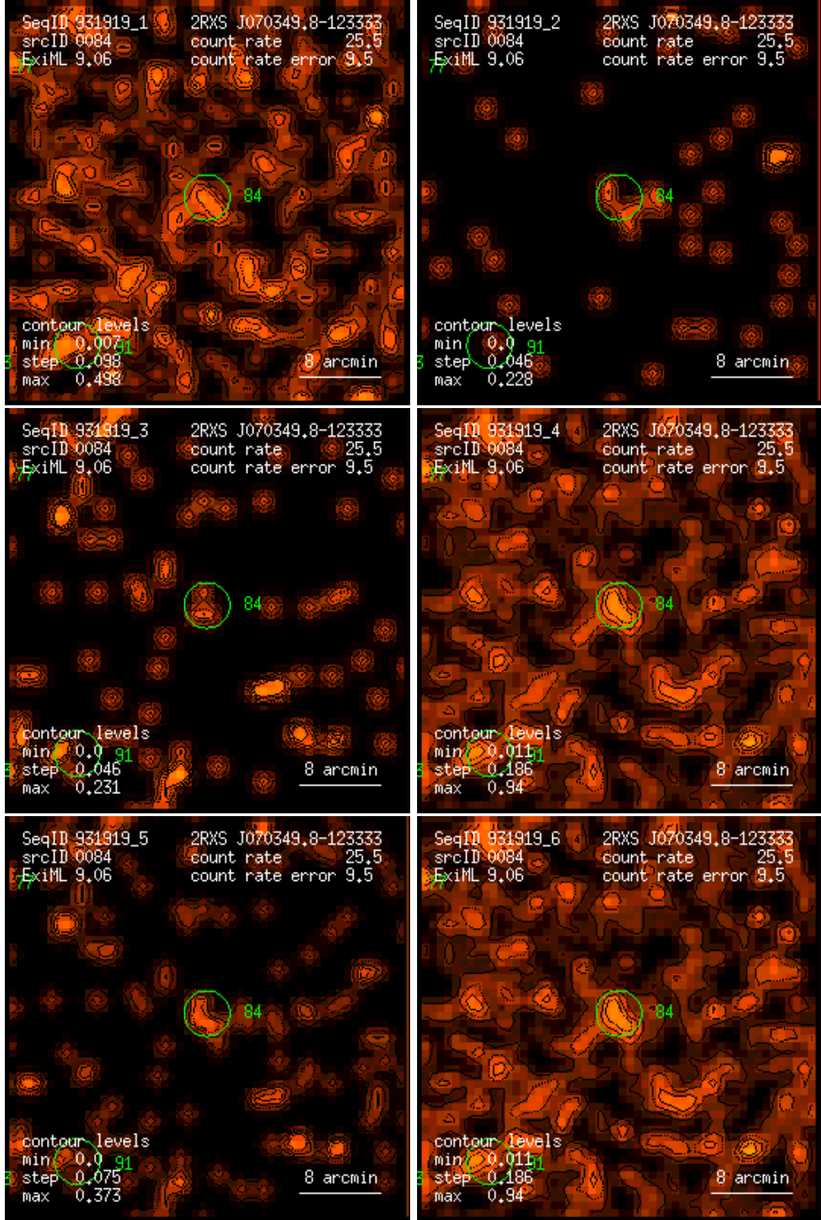
Figure 84: RASS 931919: detection 0084: band rate images, Gaussian filter: (1) PSPC channels 11 – 41, (2) 52 – 90, (3) 91 – 201, (4) 11 – 235, (5) 52 – 201, (6) 11 – 201. Broad band rates in counts/ks. Band rate contour levels in counts/ks/arcmin 2 .
