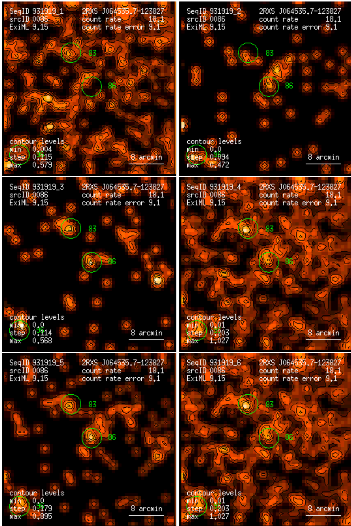
Figure 86: RASS 931919: detection 0086: band rate images, Gaussian filter: (1) PSPC channels 11 – 41, (2) 52 – 90, (3) 91 – 201, (4) 11 – 235, (5) 52 – 201, (6) 11 – 201. Broad band rates in counts/ks. Band rate contour levels in counts/ks/arcmin 2 .
