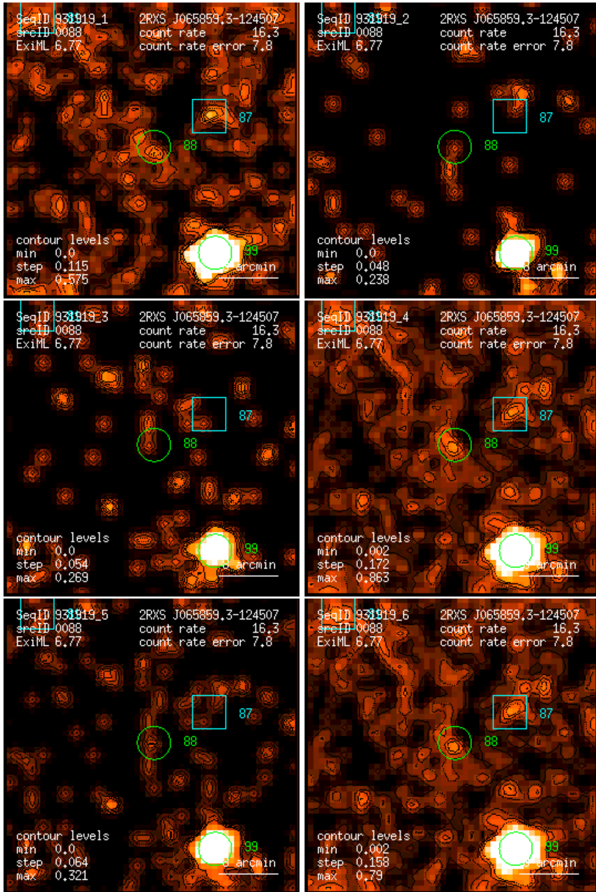
Figure 88: RASS 931919: detection 0088: band rate images, Gaussian filter: (1) PSPC channels 11 – 41, (2) 52 – 90, (3) 91 – 201, (4) 11 – 235, (5) 52 – 201, (6) 11 – 201. Broad band rates in counts/ks. Band rate contour levels in counts/ks/arcmin 2 .
