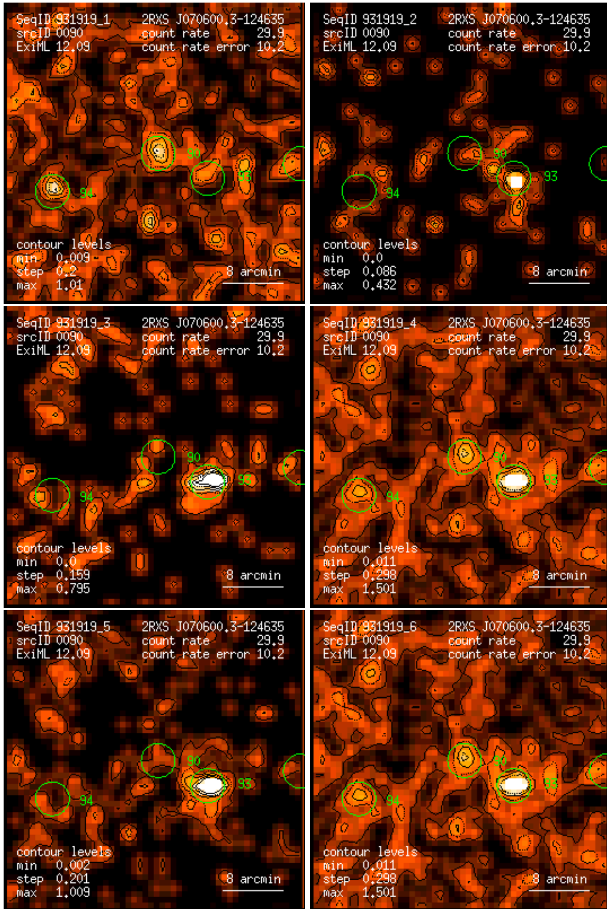
Figure 90: RASS 931919: detection 0090: band rate images, Gaussian filter: (1) PSPC channels 11 – 41, (2) 52 – 90, (3) 91 – 201, (4) 11 – 235, (5) 52 – 201, (6) 11 – 201. Broad band rates in counts/ks. Band rate contour levels in counts/ks/arcmin 2 .
